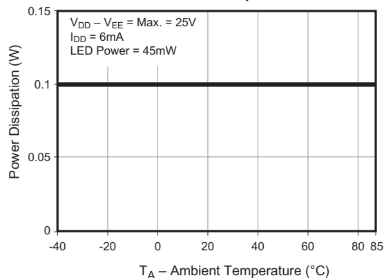
Fig. 12 Absolute Maximum Power Dissipation vs. Ambient Temperature
