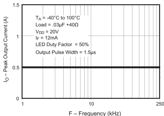
Fig. 13 Output Current Derating vs. Frequency
