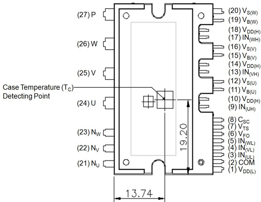
Figure 2. Top View
