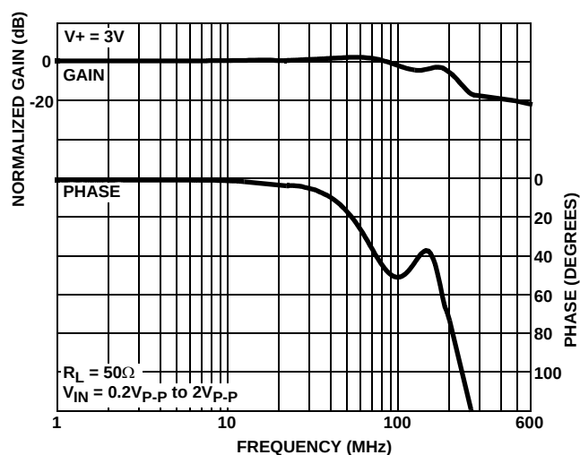
FIGURE 15. FREQUENCY RESPONSE
