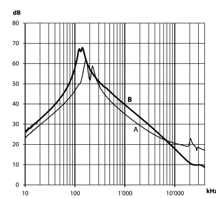
1'500/2'300 A types
