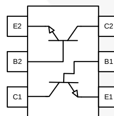
Figure 2. FFB2222A Internal Connection
