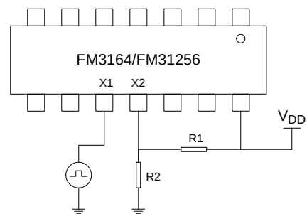
Figure 10. External Oscillator
