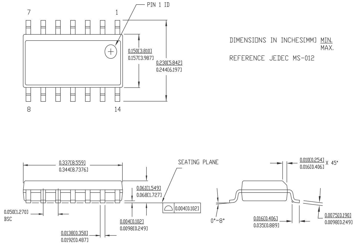
Figure 27. 14-pin SOIC (150 Mils) Package Outline, 51-85067
