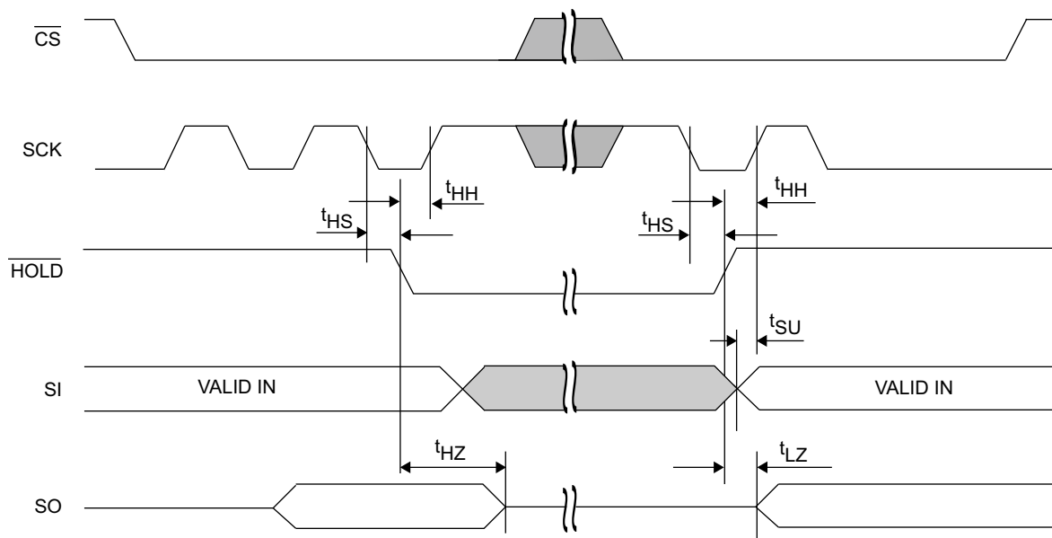
Figure 17. HOLD Timing
