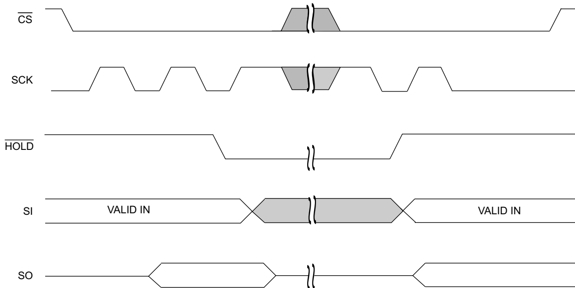
Figure 13. HOLD Operation [2]
