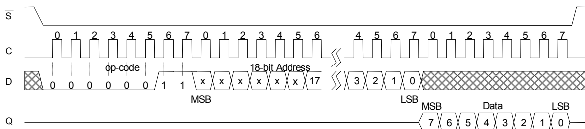
Figure 10. Memory Read
