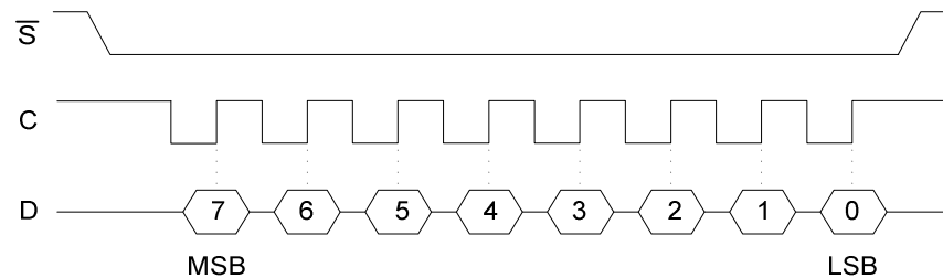
Figure 4. SPI Modes 0 & 3
