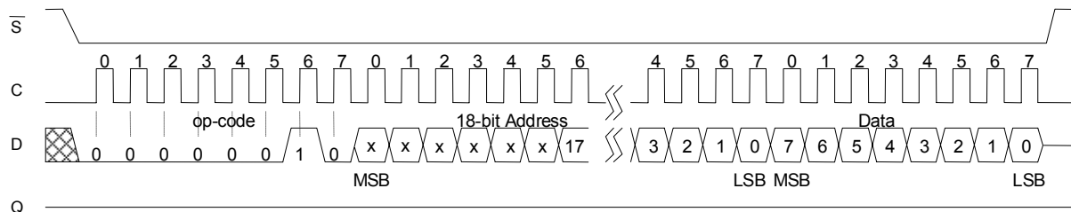
Figure 9. Memory Write
