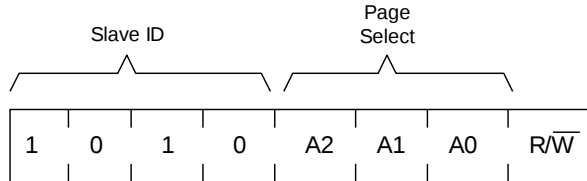
Figure 4. Slave Address
