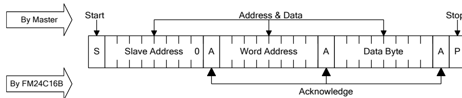
Figure 5. Single Byte Write
