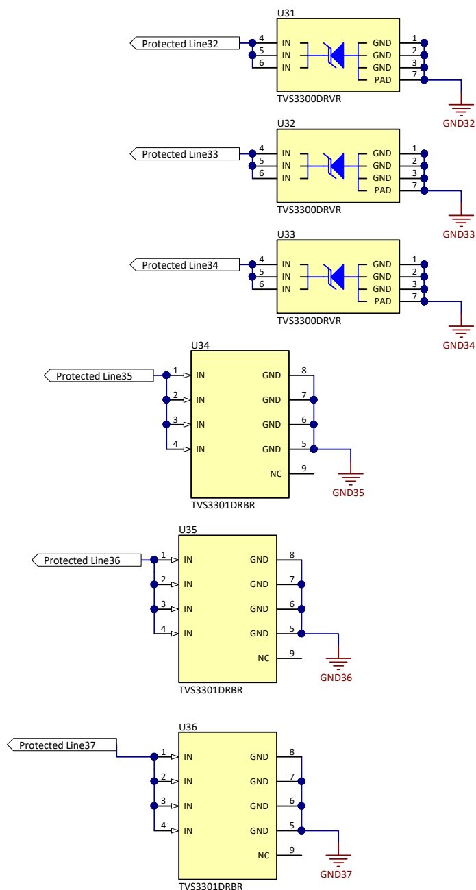
Figure 12. TVS330X Schematic
