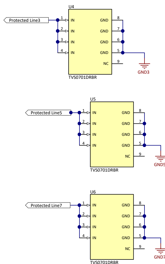
Figure 7. TVS0701 Schematic
