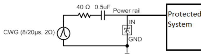
Figure 3. Surge Test Setup Unidirectional Configuration
