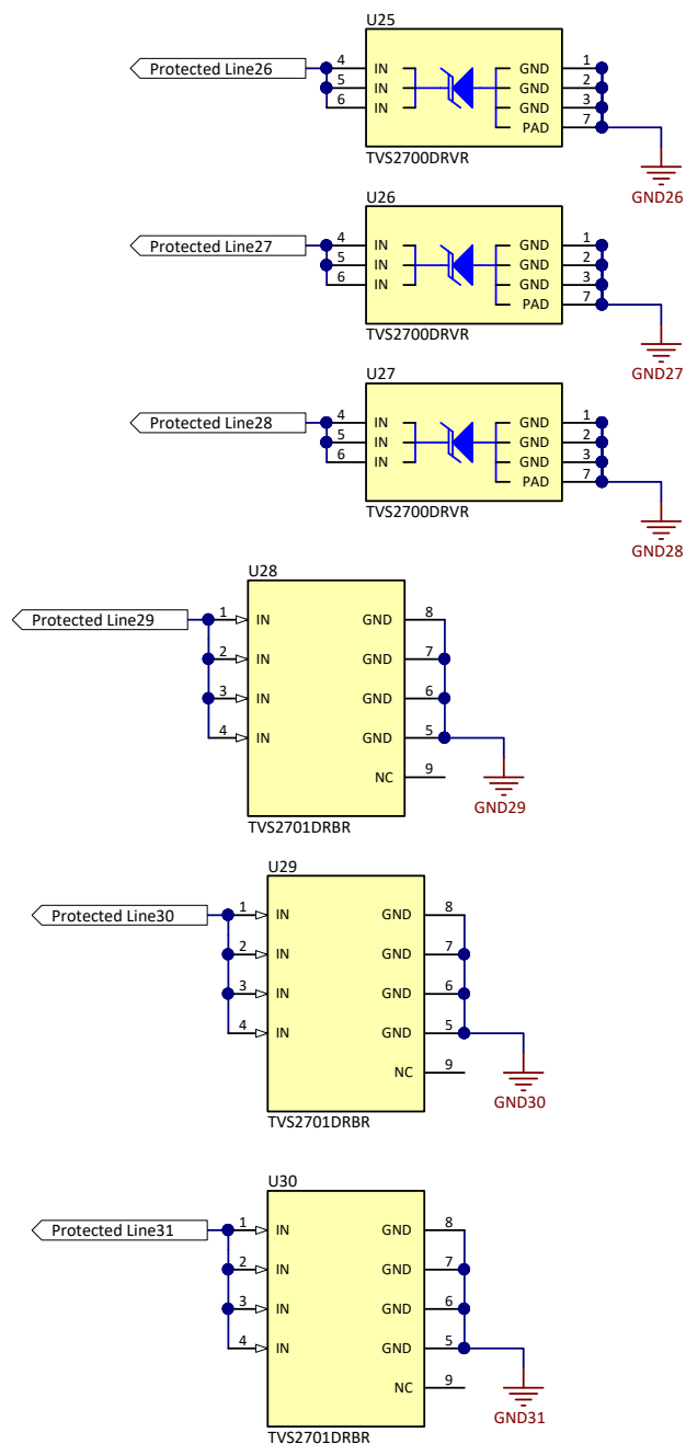
Figure 11. TVS270X Schematic
