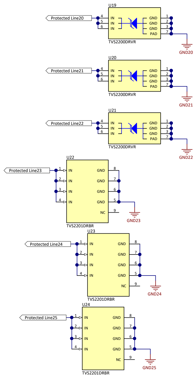
Figure 10. TVS220X Schematic
