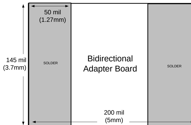
Figure 2. Bidirectional Adapter Board
