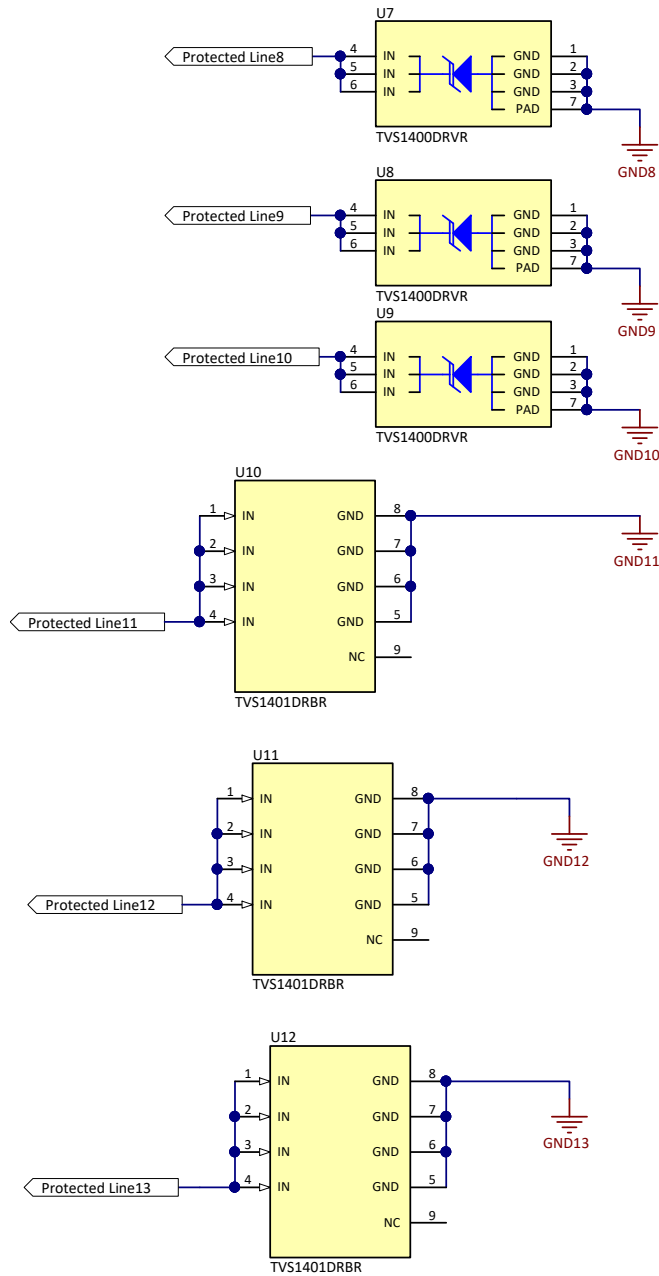
Figure 8. TVS140X Schematic
