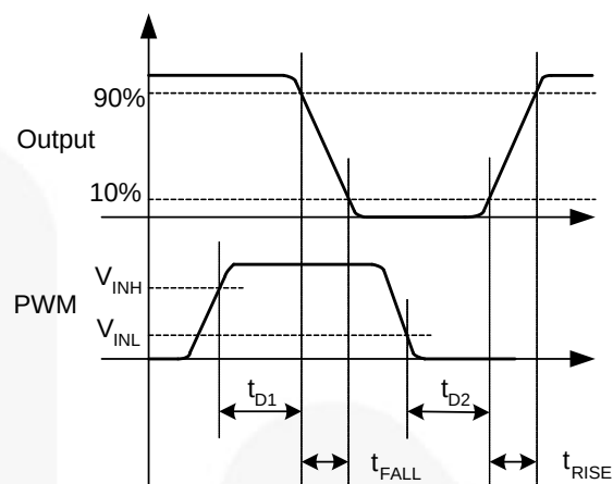
Figure 7. DIM Pin
