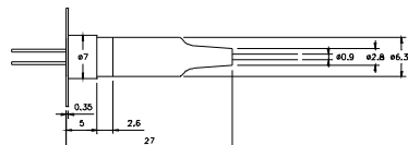
VERTICAL FLANGE
