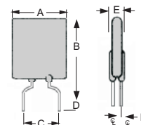
Figure 2 Lead Size: 20AWG Ø 0.81 mm Diameter
