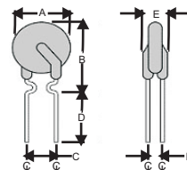
Figure 1 Lead Size: 24AWG Ø 0.51 mm Diameter
