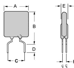
Fig.4 Lead Size : 18AWG Φ 1.00 mm Diameter
