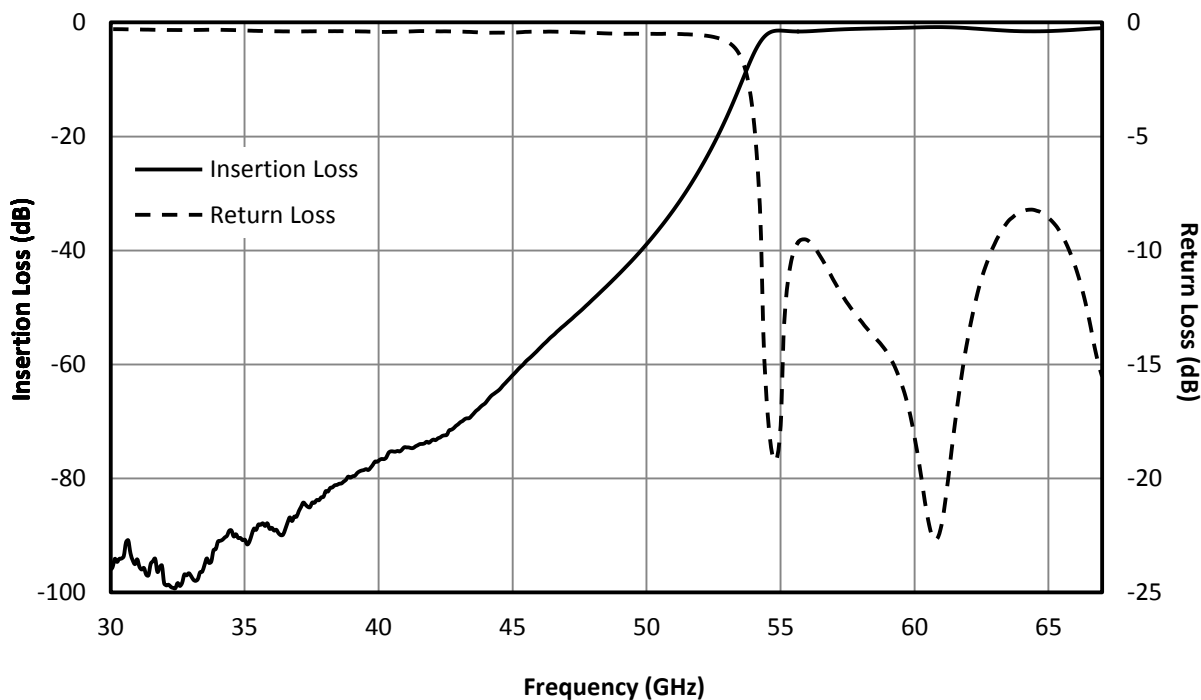
Fig. 1. Magnitude response for a typical FH-5500 Filter.
