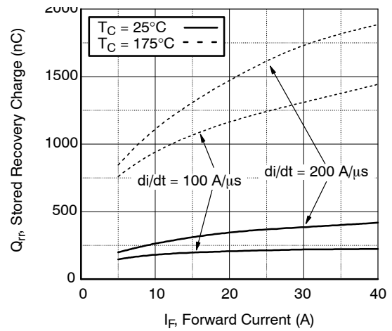
Figure 20. Stored Charge
