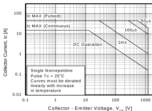
Figure 14. SOA Characteristics
