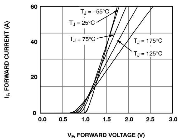
Figure 1. Forward Characteristics
