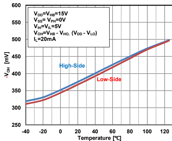
Figure 26. High-Level Output Voltage Deviation from the V_{\text{BH}}(V_{\text{DD}}) vs. Temp.
