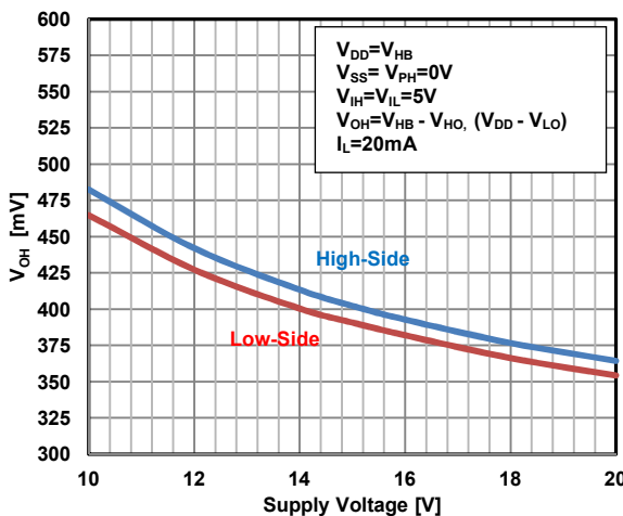
Figure 25. High-Level Output Voltage Deviation from the V_{\text{BH}}(V_{\text{DD}}) vs. Supply Voltage ( V_{\text{DD}} )
