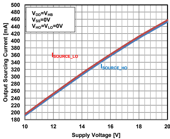
Figure 21. Output Sourcing Current vs. Supply Voltage ( V_{\text{DD}} )
