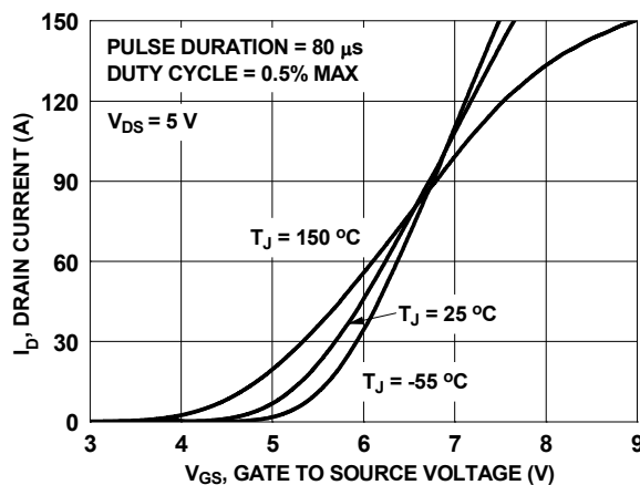
Figure 42. Transfer Characteristics
