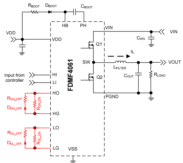
Figure 68. Gate driver resistor-diode circuit
