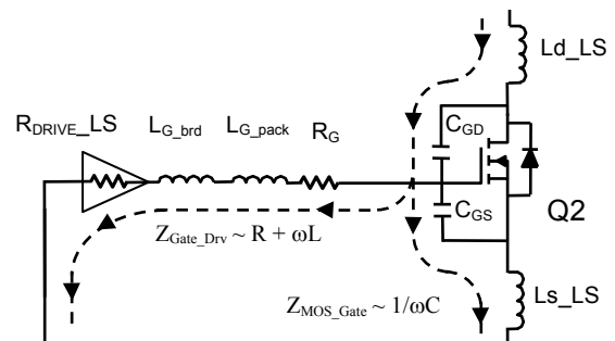
Figure 69. C_{GD} \times dV_{DS}/dt current flow
