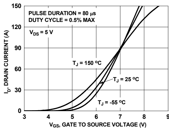
Figure 54. Transfer Characteristics
