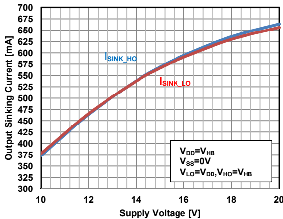
Figure 23. Output Sinking Current vs. Supply Voltage ( V_{\text{DD}} )
