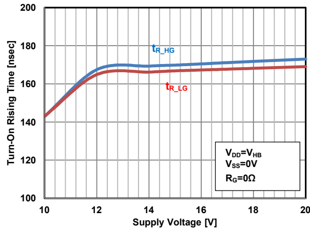
Figure 17. Turn-On Rising Time vs. Supply Voltage ( V_{DD} )
