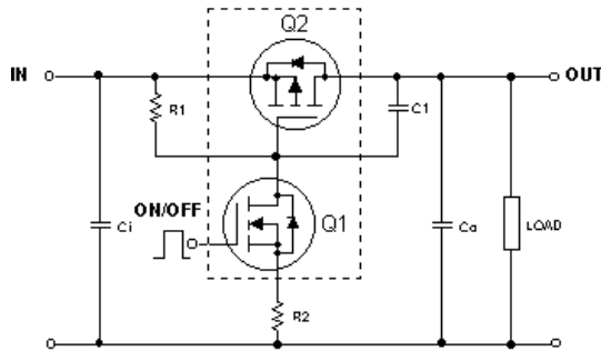
APPLICATION CIRCUIT
