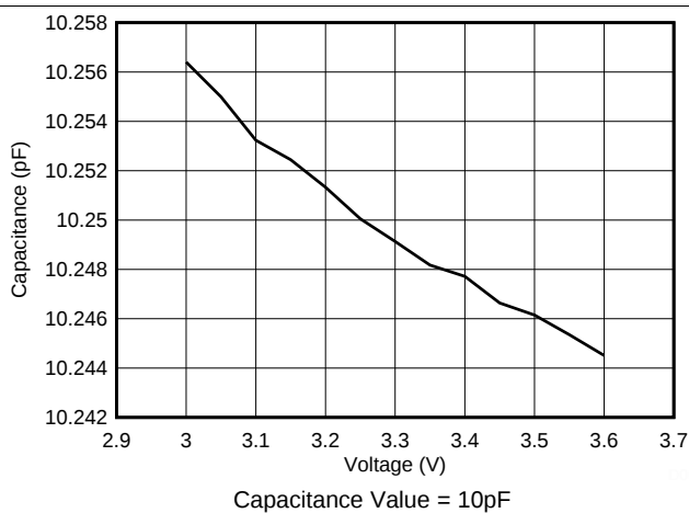
Figure 6. Capacitance vs Voltage
