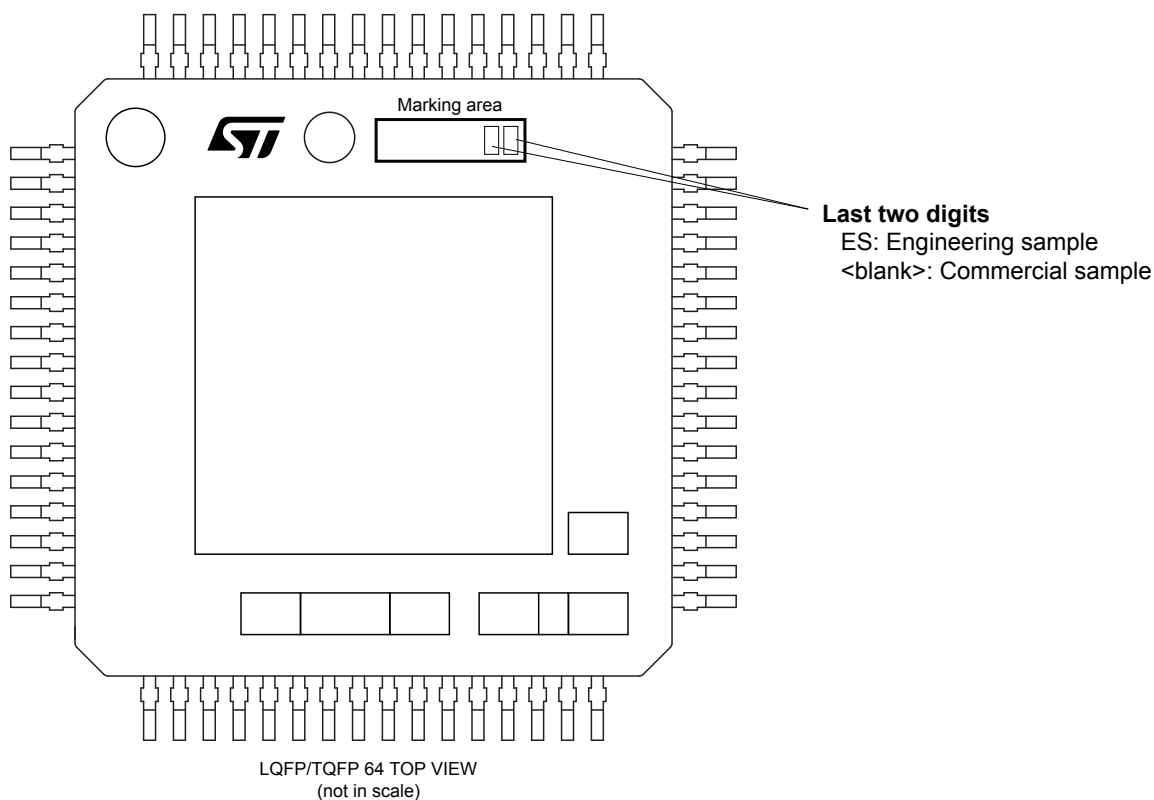
Figure 5. LQFP64 (10x10x1.4 mm exp. pad up) marking information
