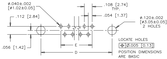
RECOMMENDED P.C.B. LAYOUT (COMPONENT SIDE OF BOARD)
