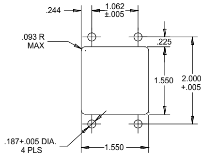
Mounting Layout
