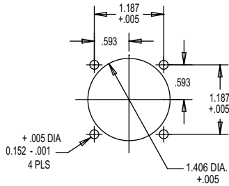
Mounting Layout
