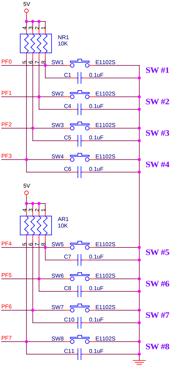
Switch Part
