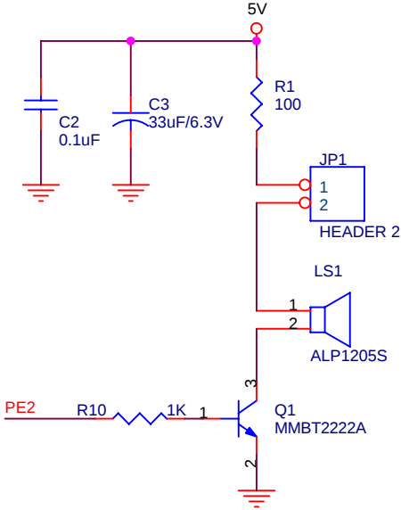
Buzzer Part
