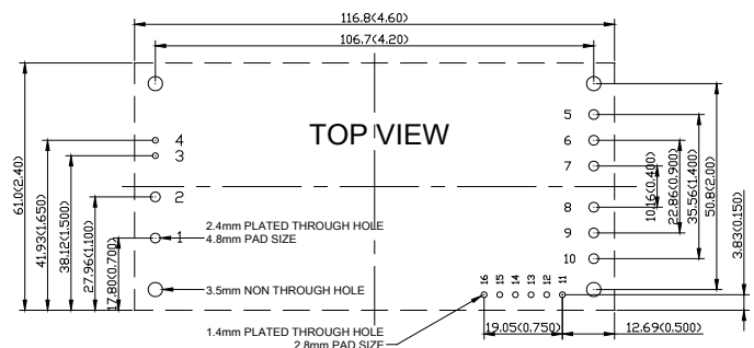
Recommend PCB Pad layout
