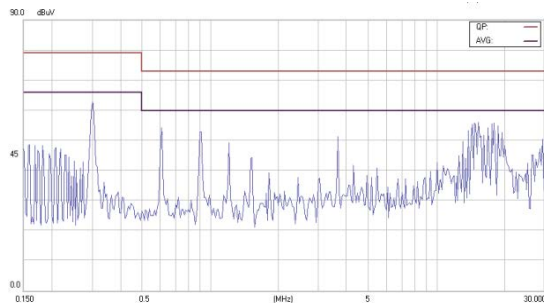
Class A test conducted for FB48S32-19
