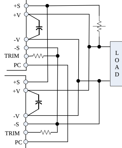
(c) N+1 redundant connection
