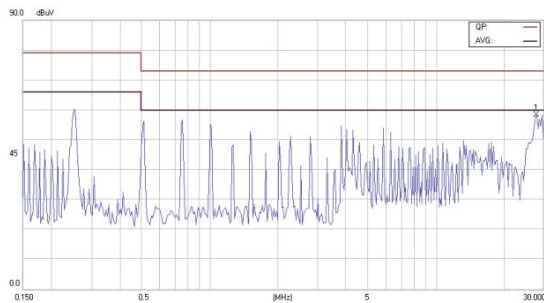
Class A test conducted for FB48S24-25
