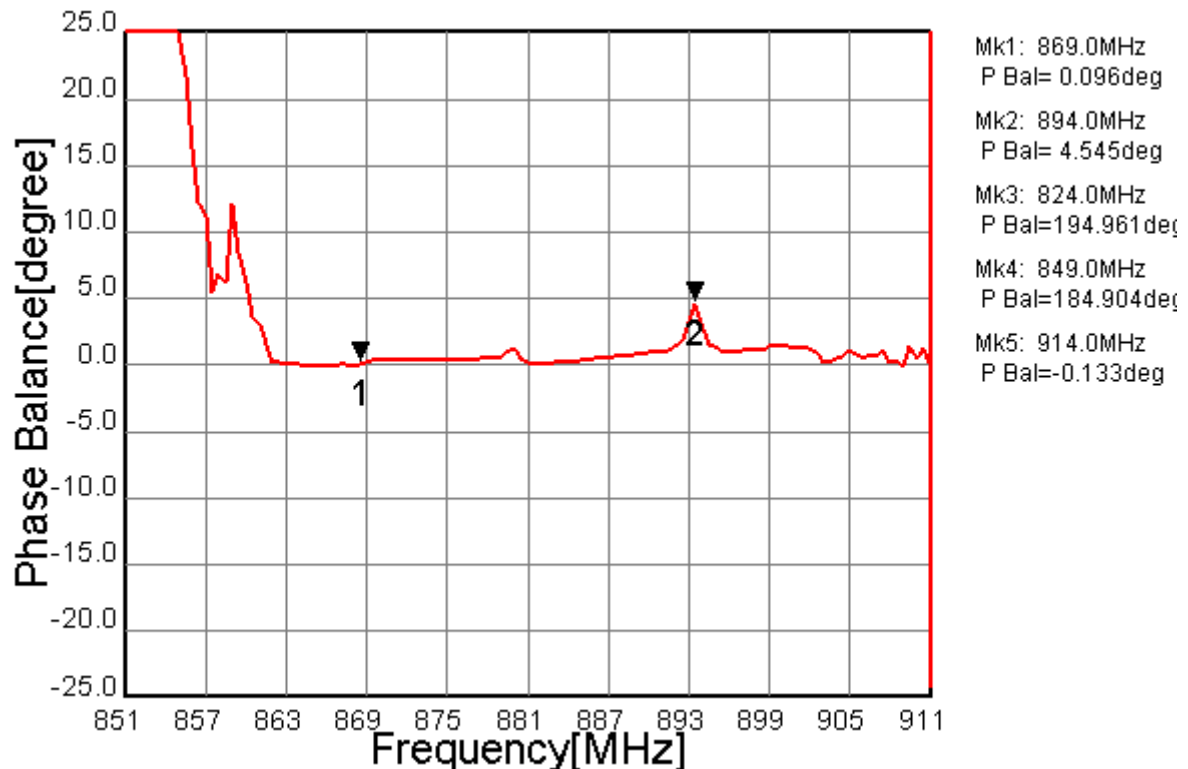
Fig.8 Phase Balance (Filter1)
