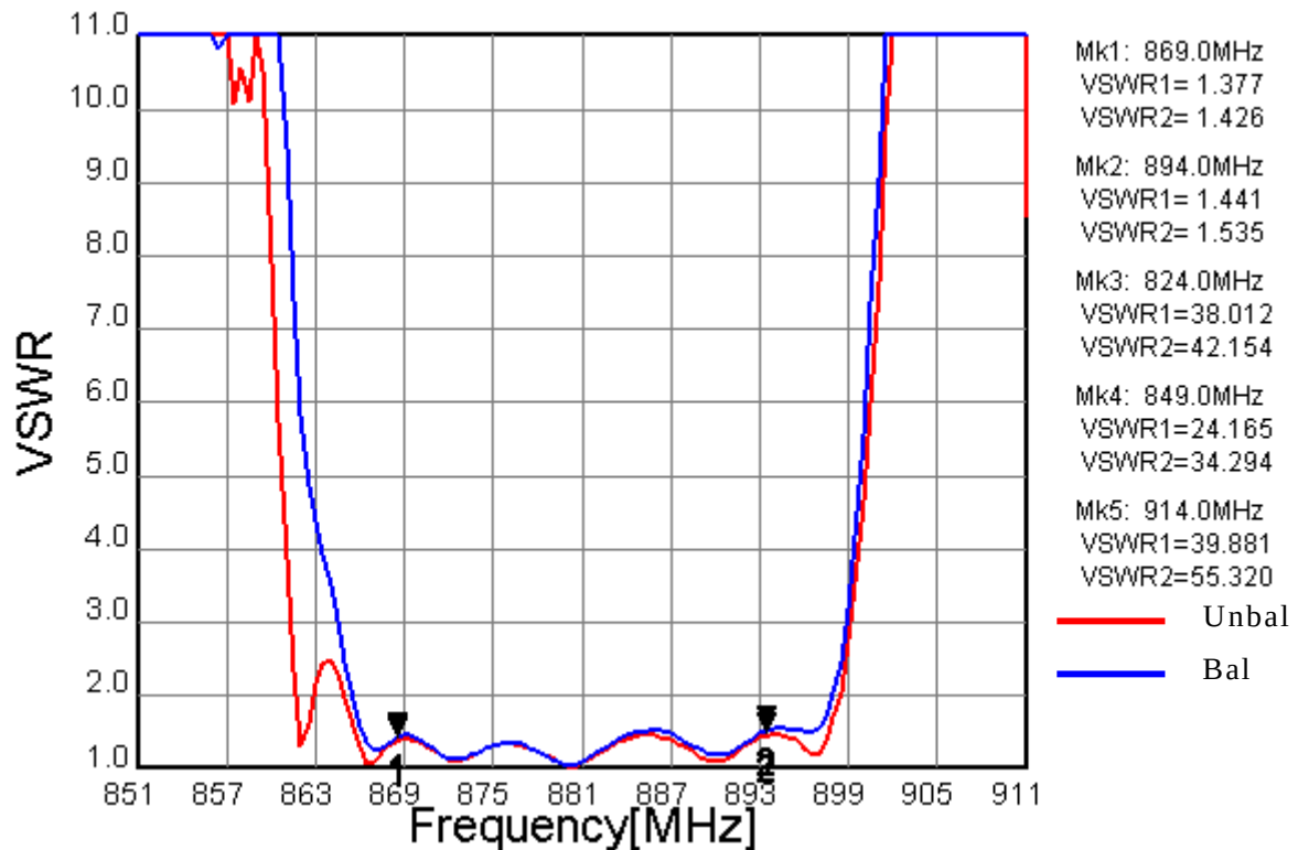
Fig.2 VSWR (Filter1)
