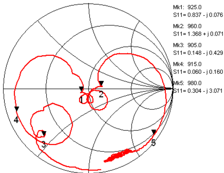
Fig.5 Impedance (S11)
