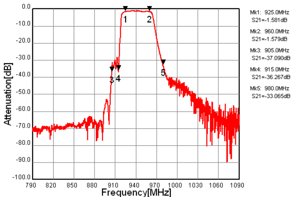
Fig.1 Pass-band Characteristic
