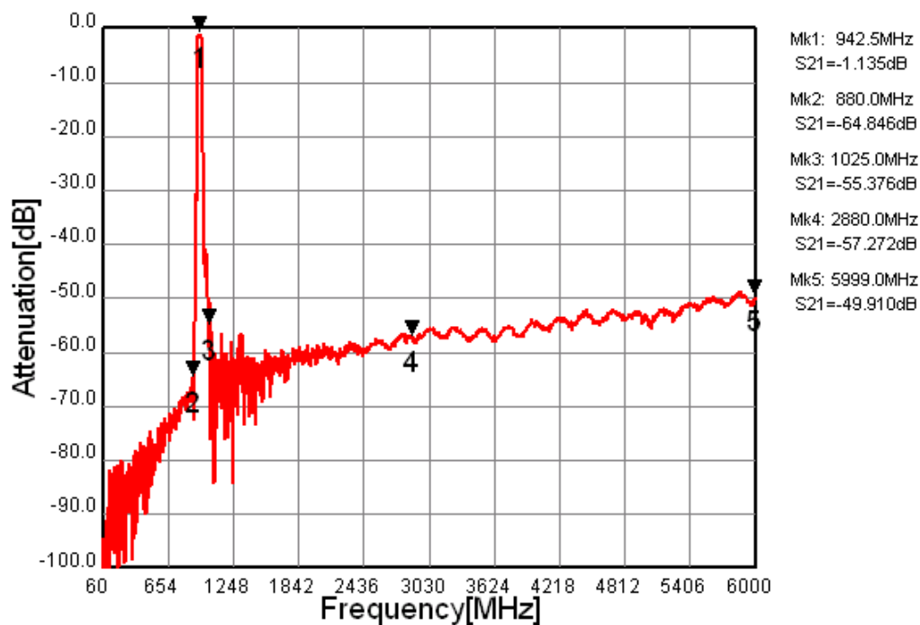
Fig.4 Wide-band Characteristic
