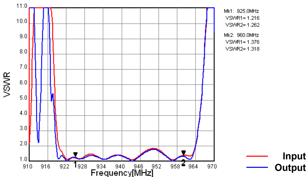
Fig.2 VSWR
