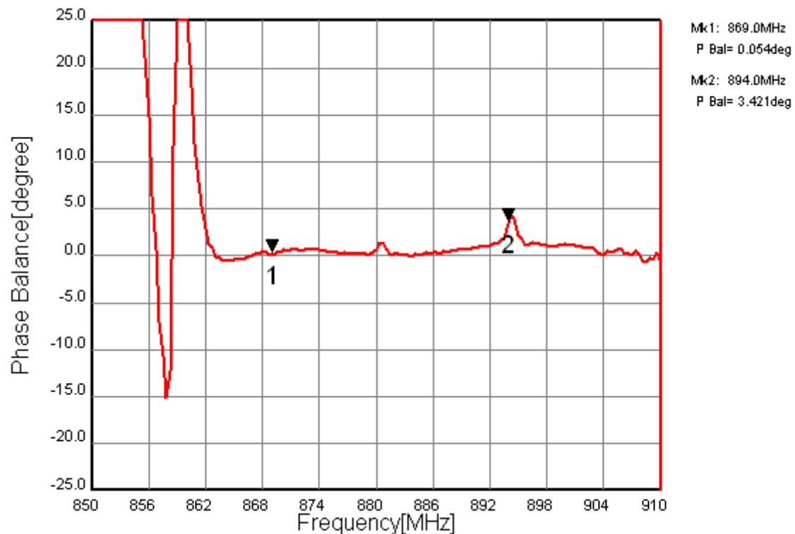
Fig.8 Phase Balance
