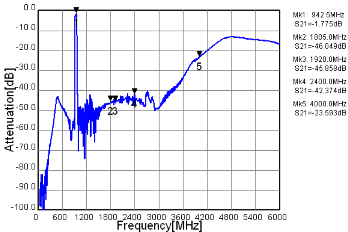
Figure 3-6. Electrical Characteristics
