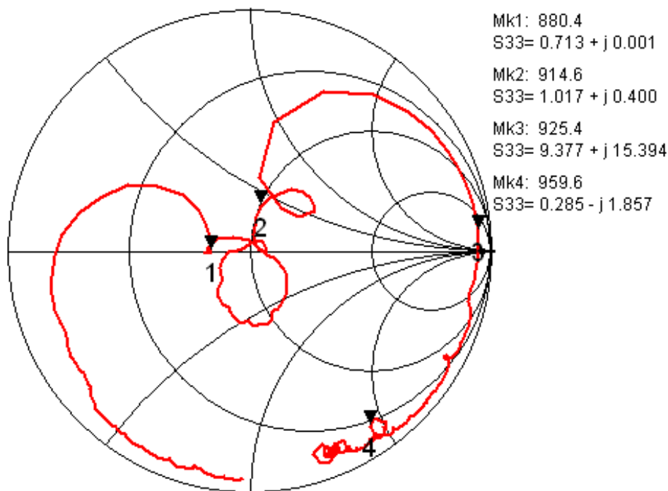
Figure 3-3. Electrical Characteristics
