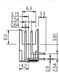
Type 02 - Right angle solder dip terminal
