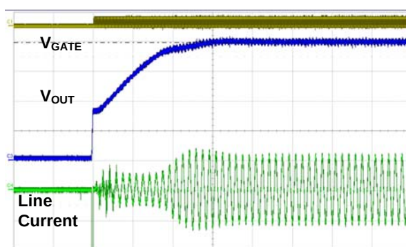
Figure 60. Full-Load Startup at 115 V AC
