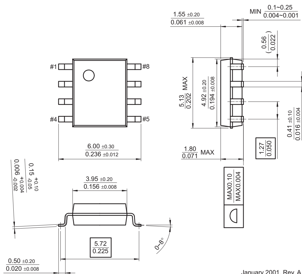
Figure 27. 8-Lead Small Outline Package (SOP)
