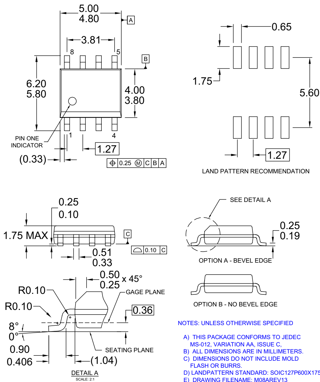
Figure 24. 8-Lead Small Outline Package (SOP)
