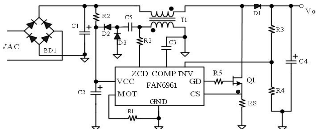
Figure 1. Typical Application
