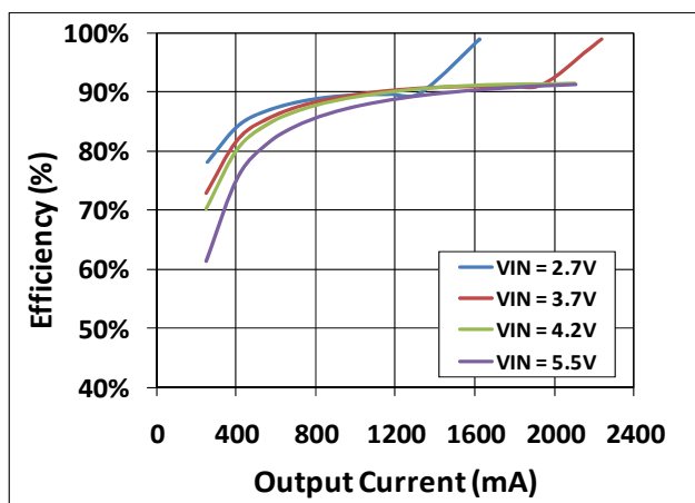
Figure 5. High-Power PWM Mode Efficiency vs. Output Current vs. Input Voltage, f_{SW} = 3\text{ MHz} , R_{PA} = 1.5\text{ }\Omega
