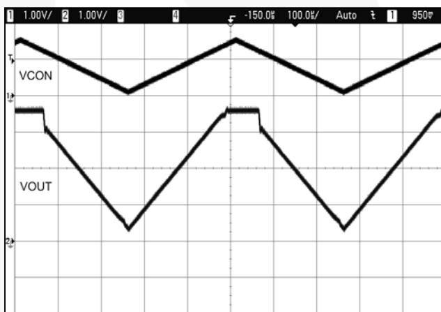
Figure 43. V_{OUT} Transient and Bypass Response \Delta V_{OUT} > 3\text{ V} , V_{CON} Stepped Above 1.5\text{ V}
