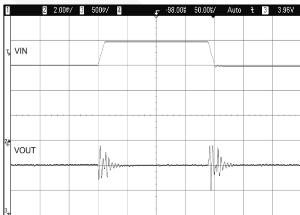
Figure 20. Line Transient V_{IN} = 3.7\text{ V} to 4.2 V, V_{OUT} = 1.0\text{ V} , 5 \Omega Load, 50 \mu\text{s}/\text{div} .
