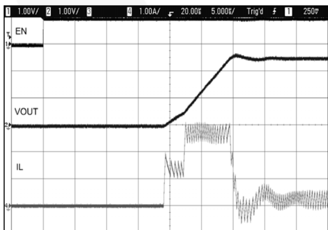
Figure 44. Soft-Start Transient Response from 0\text{ mA} to 100\text{ mA} in High-Power Mode
