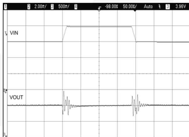
Figure 21. Line Transient V_{IN} = 3.7\text{ V} to 4.2 V, V_{OUT} = 2.5\text{ V} , 5 \Omega Load, 50 \mu\text{s}/\text{div} .
