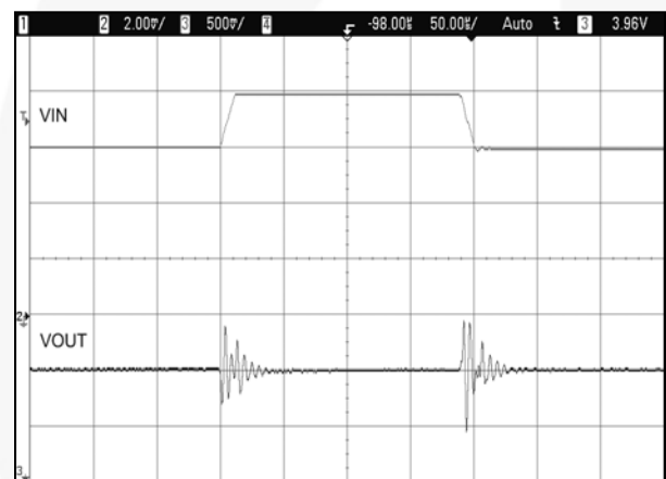
Figure 18. Line Transient V_{IN} = 3.7\text{ V} to 4.2 V, V_{OUT} = 1.0\text{ V} , 10 \Omega Load, 50 \mu\text{s}/\text{div} .
