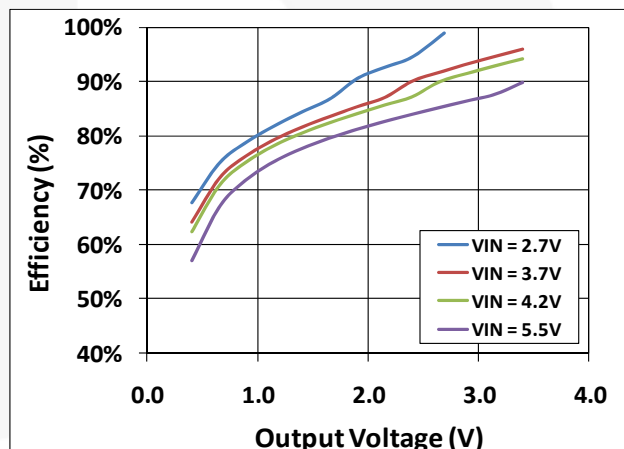
Figure 14. Low-Power Auto Mode Efficiency vs. Output Voltage vs. Input Voltage, f_{SW} = 6\text{ MHz} , R_{PA} = 10.0\text{ }\Omega
