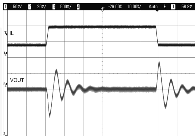
Figure 29. Load Transient, 200 mA to 800 mA, V_{OUT} = 2.5\text{ V} in Low-Power Mode
