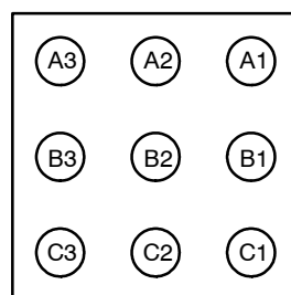
Figure 4. Bottom View
