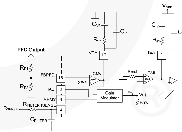
Figure 46. Compensation Network Connection for the Voltage and Current Error Amplifiers
