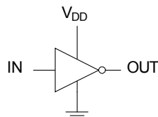
Figure 49. Inverting Configuration
