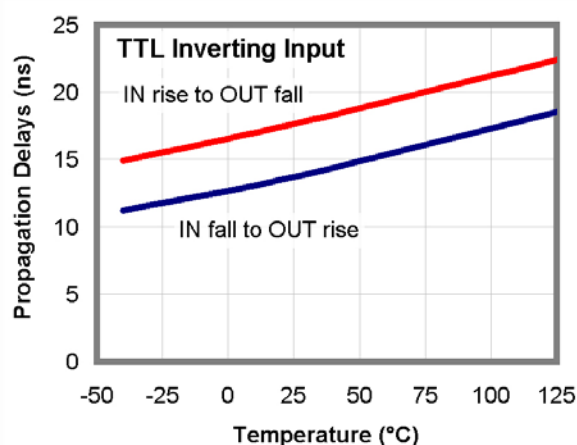
Figure 31. Propagation Delay vs. Temperature
