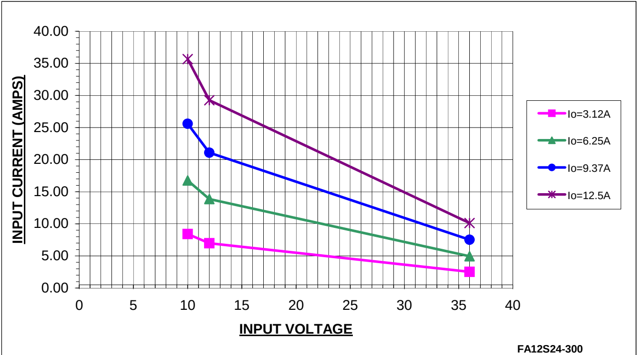
Graph 3: Input Current vs. Input Voltage
