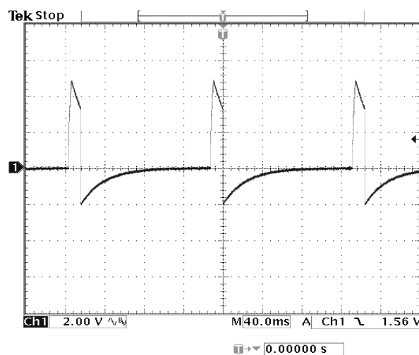
Photo 8: Overload output current, 0.2 Ohm impedance. 24Vin, 10A / div.
