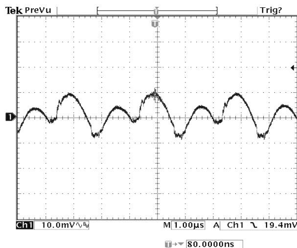
Photo 4: Output ripple, 10Vin, full load. 10mV / div.
