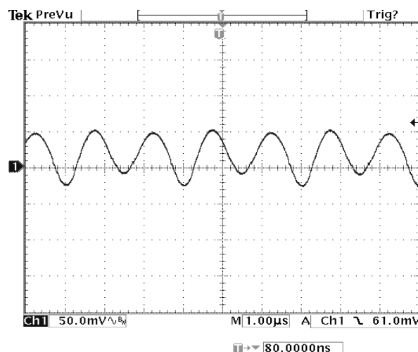
Photo 6: . Output ripple, 36Vin, full load. 50mV / div.
