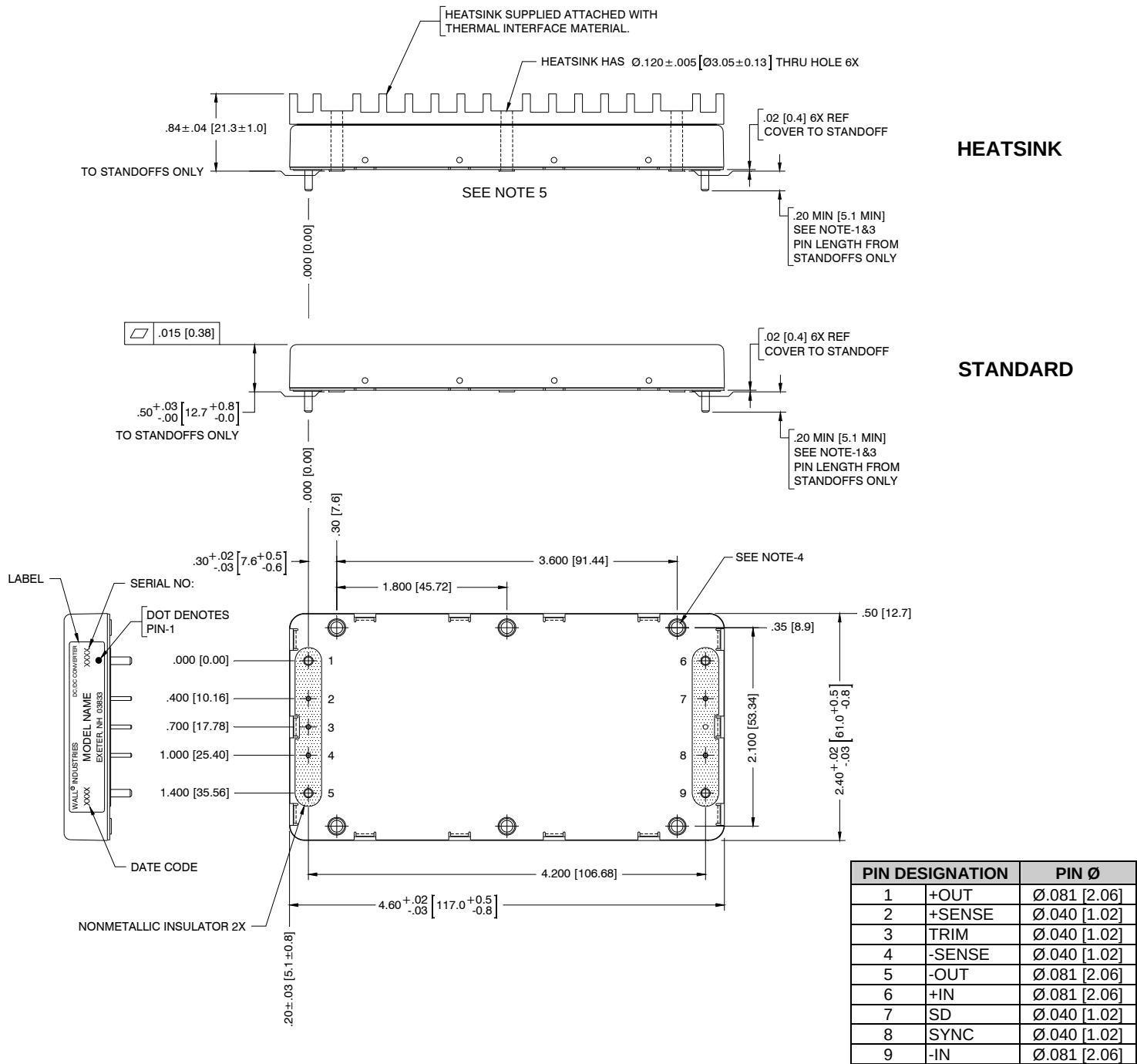
Figure 1: Mechanical Dimensions
