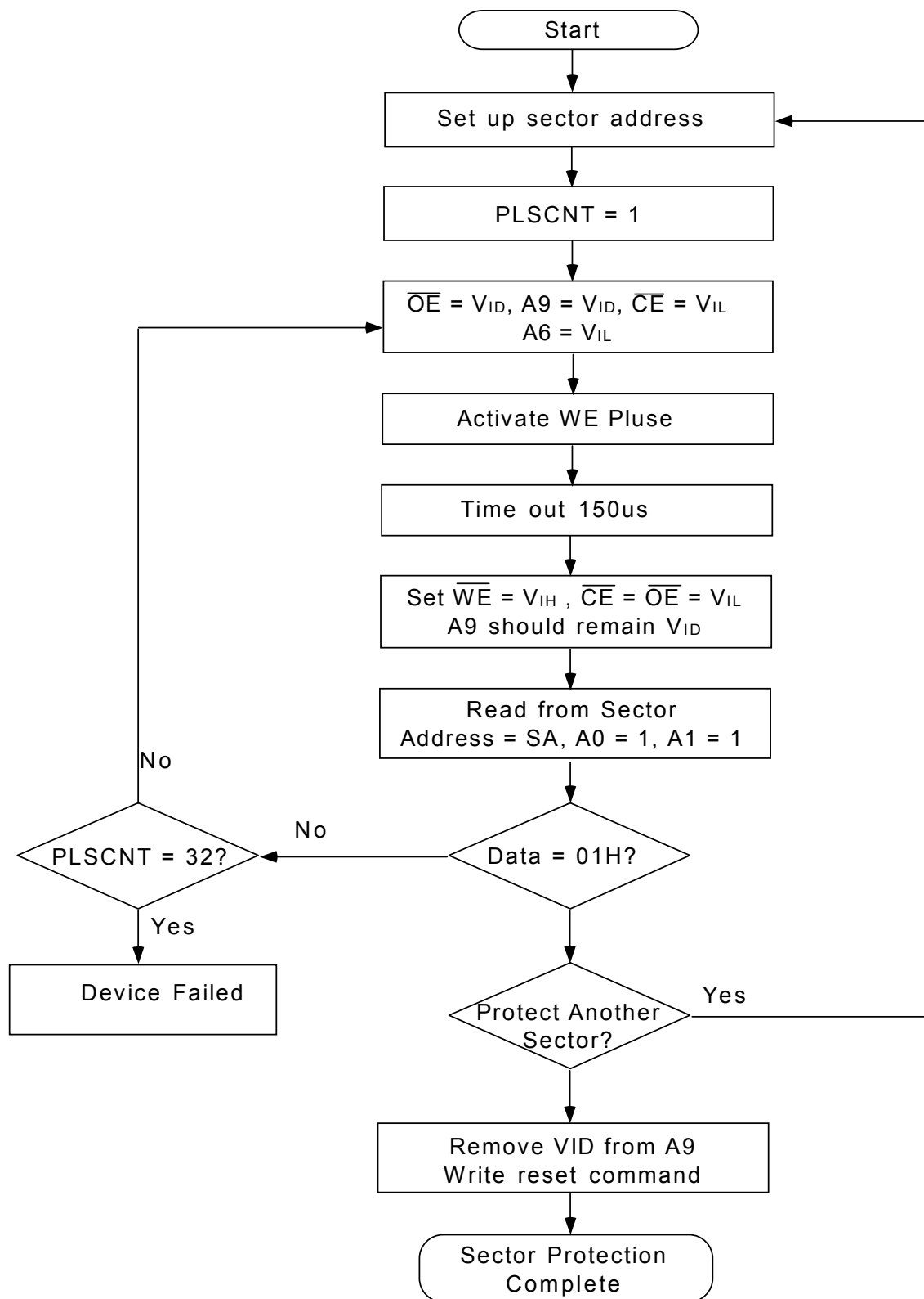
Figure 18. Sector Protection Algorithm (A9, \overline{\text{OE}} Control)
