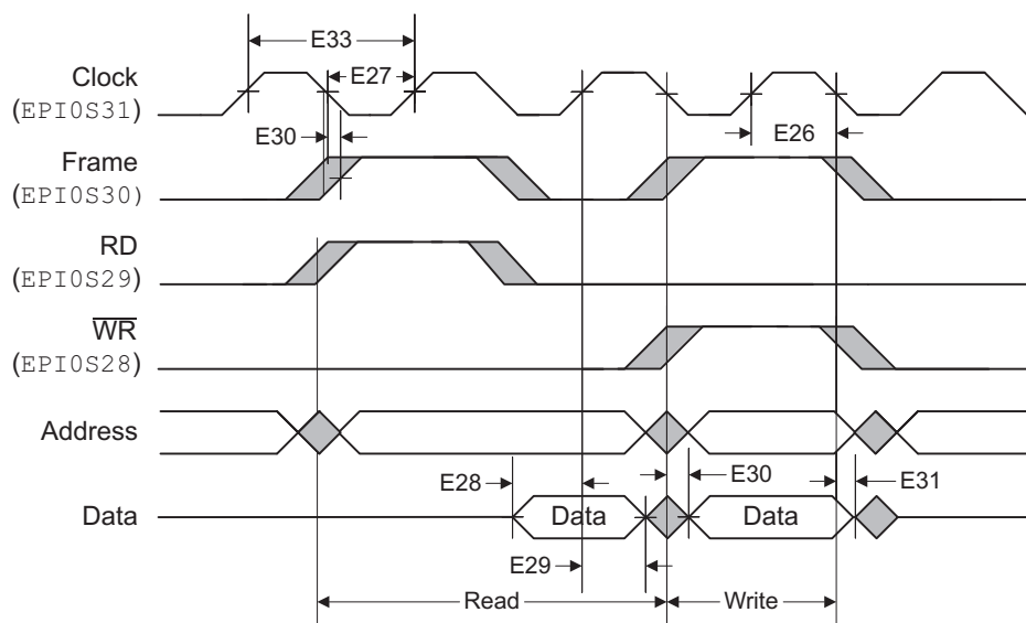
Figure 5-28. General-Purpose Mode Read and Write Timing
