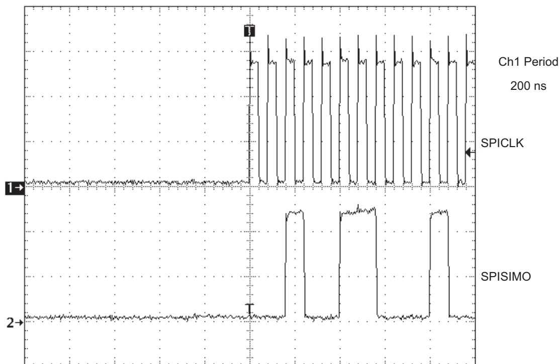
Figure 12-25. CLOCK POLARITY = 0, CLOCK PHASE = 0 (All data transitions are during the rising edge, non-delayed clock. Inactive level is low.)
