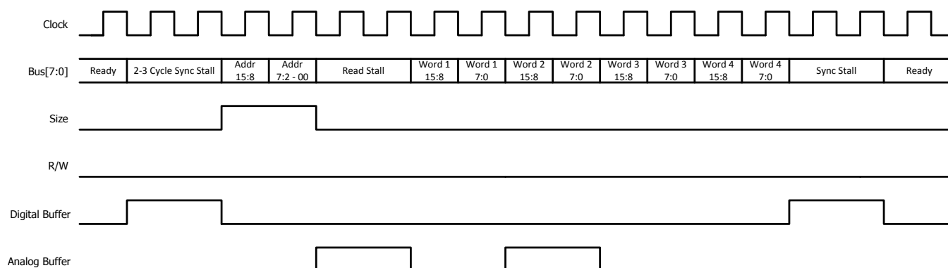
Figure 10-7. 64-bit Read
