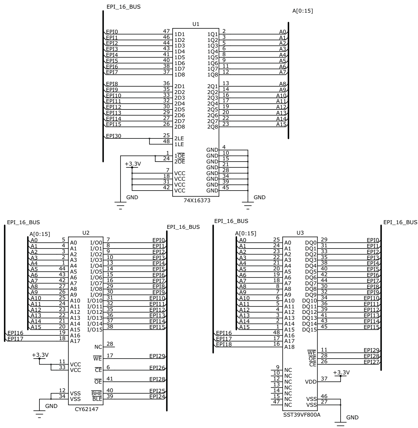
Figure 17-7. Example Schematic for Muxed Host-Bus 16 Mode
