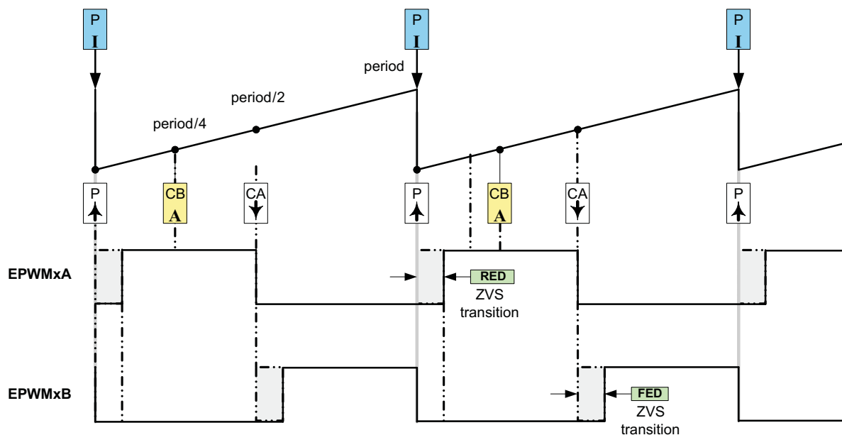
Figure 7-74. H-Bridge LLC Resonant Converter PWM Waveforms
