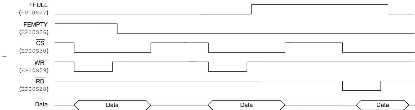
Figure 17-14. Two-Entry FIFO
