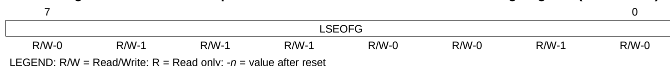
Figure 18-26. USB Low-Speed Last Transaction to End of Frame Timing Register (USBLSEOF)
