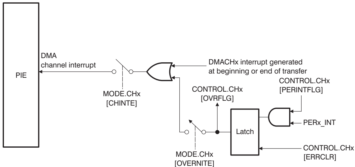
Figure 11-7. Overflow Detection Logic
