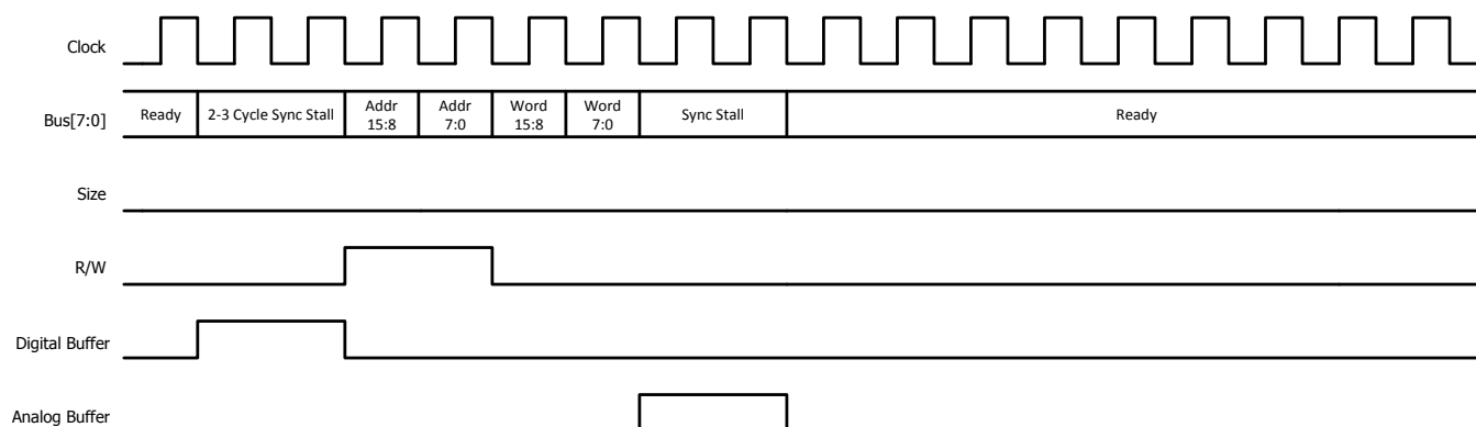
Figure 10-3. 16-bit Write
