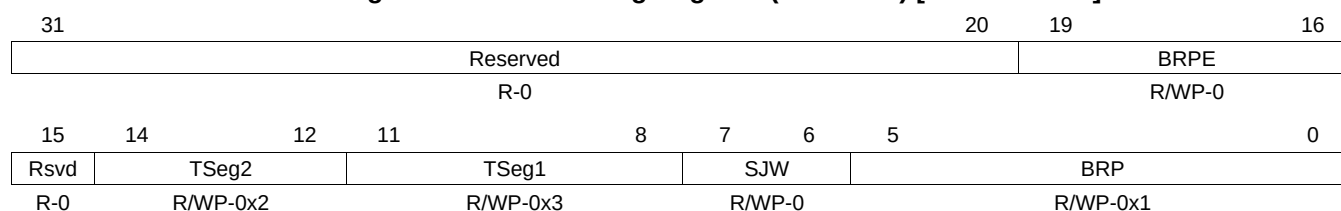
Figure 23-22. Bit Timing Register (CAN BTR) [offset = 0x0C]
