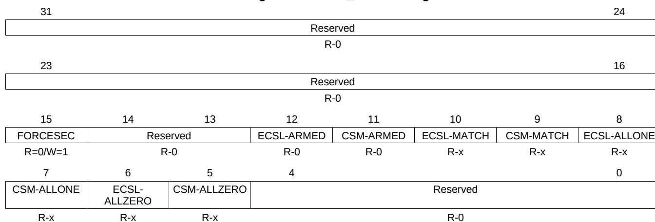
Figure 1-145. Z2_CSMCR Register
