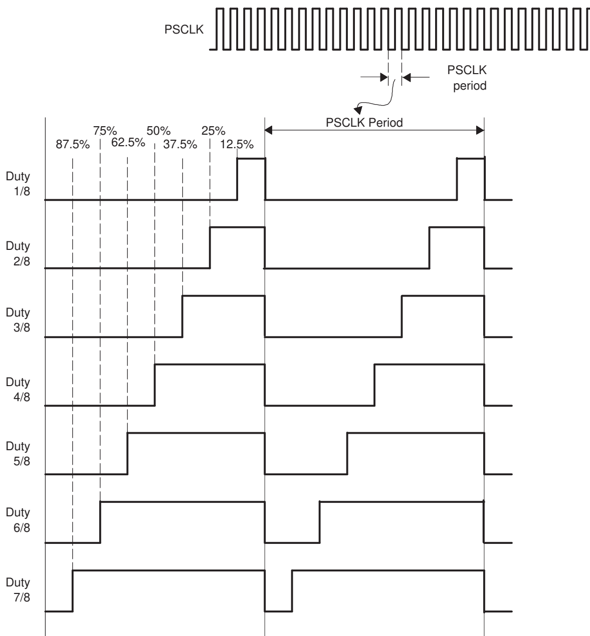
Figure 7-37. PWM-Chopper Submodule Waveforms Showing the Pulse Width (Duty Cycle) Control of Sustaining Pulses
