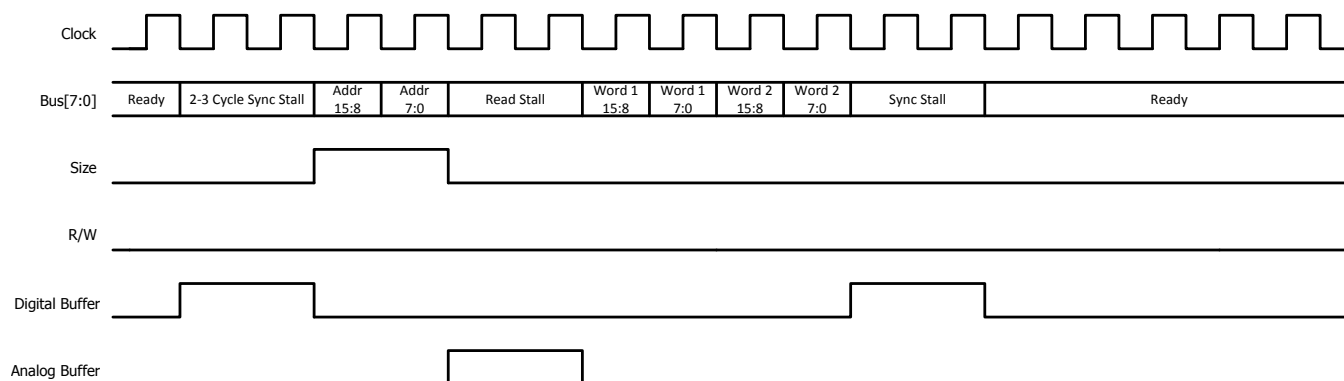
Figure 10-6. 32-bit Read
