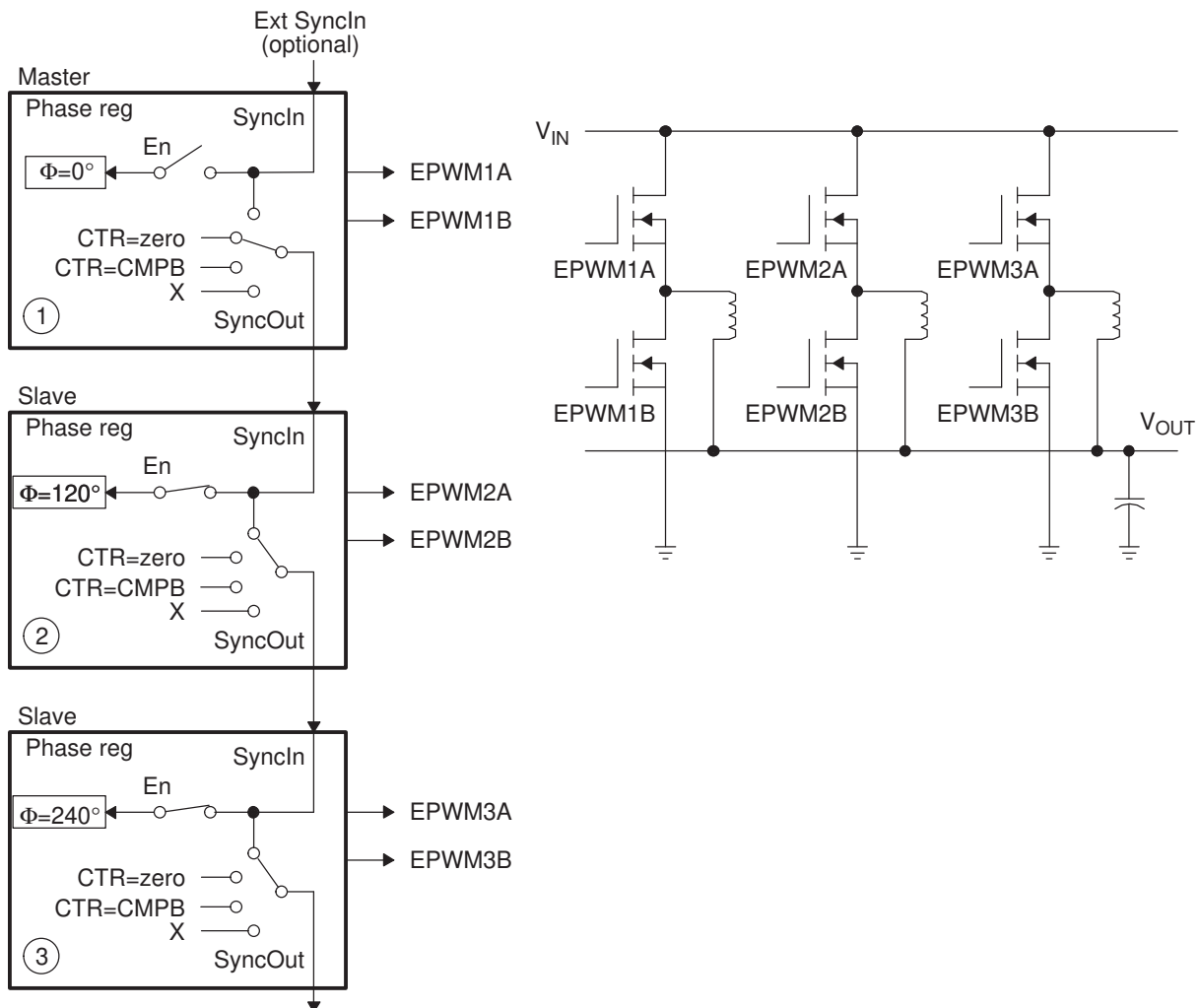
Figure 7-67. Control of a 3-Phase Interleaved DC/DC Converter
