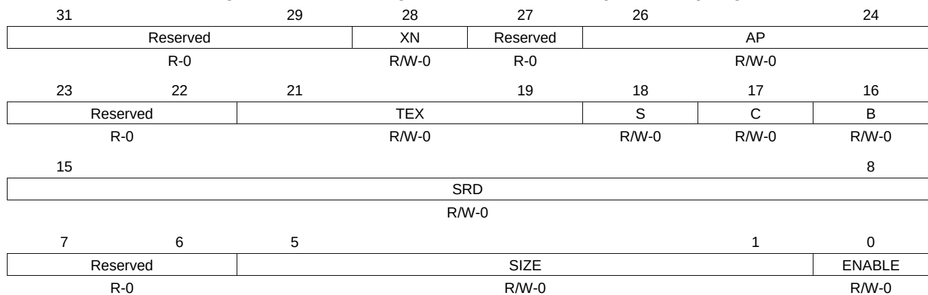
Figure 25-51. MPU Region Attribute and Size (MPUATTR) Register
