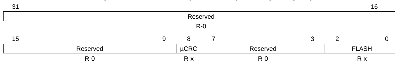
Figure 1-37. Master Subsystem Configuration (MCNF) Register
