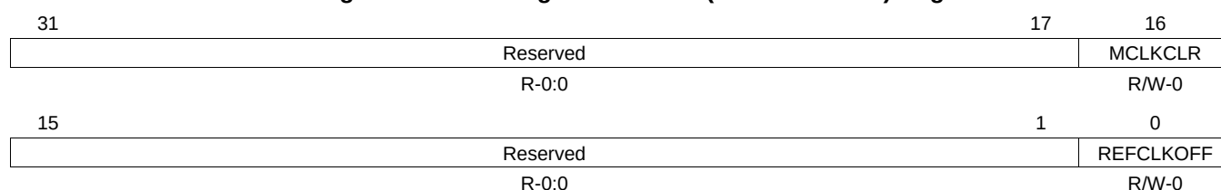
Figure 1-91. Missing Clock Force (MCLKFRCCLR) Register
