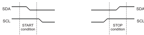
Figure 22-3. START and STOP Conditions
