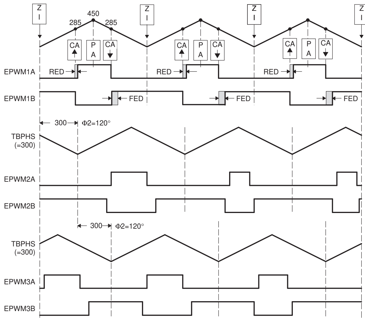
Figure 7-68. 3-Phase Interleaved DC/DC Converter Waveforms for Figure 7-67
