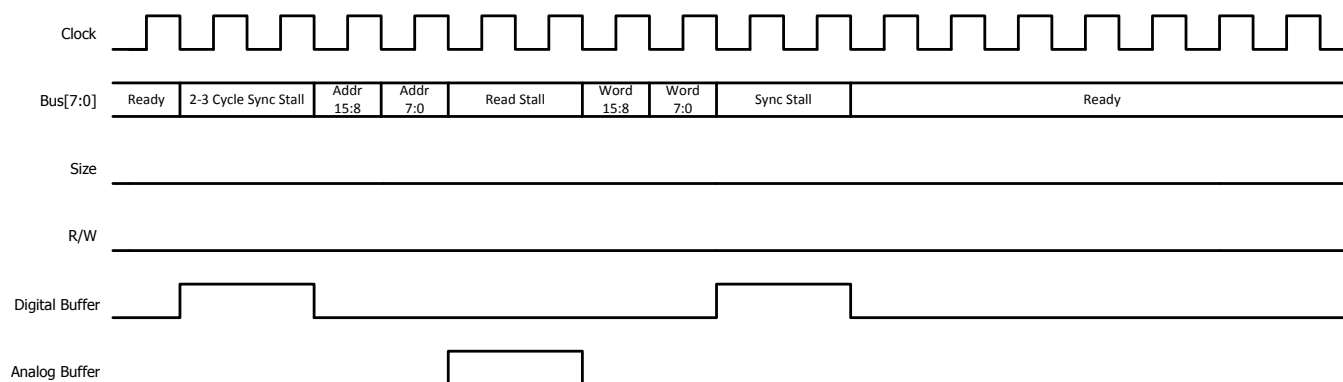
Figure 10-5. 16-bit Read
