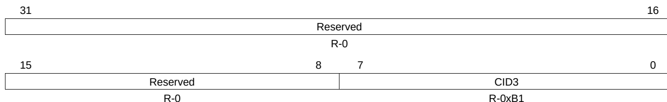
Figure 4-34. GPIO PrimeCell Identification 3 (GPIOPCellID3) Register
