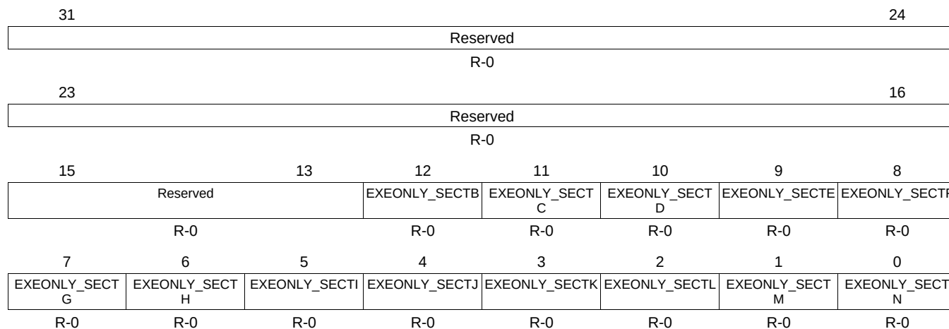
Figure 1-150. Z1_EXEONLYR Register
