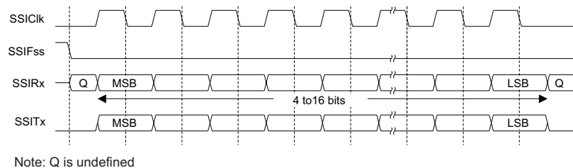
Figure 20-6. Freescale SPI Frame Format with SPO =0 and SPH=1
