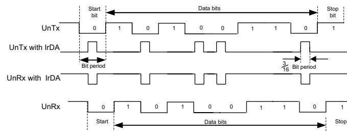
Figure 21-3. IrDA Data Modulation
