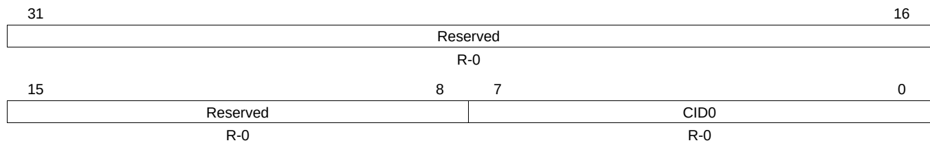
Figure 4-31. GPIO PrimeCell Identification 0 (GPIOCellID0) Register
