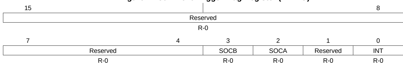
Figure 7-136. Event-Trigger Flag Register (ETFLG)
