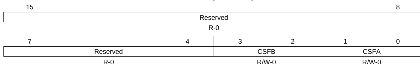
Figure 7-102. Action-Qualifier Continuous Software Force Register and Mirror Register (AQCSFRC / AQCSFRCM)
