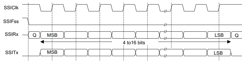
Figure 20-9. Freescale SPI Frame Format with SPO =1 and SPH =1
