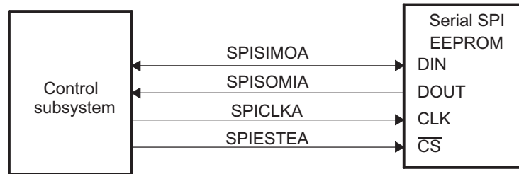
Figure 6-20. SPI Loader
