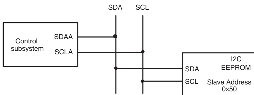
Figure 6-23. EEPROM Device at Address 0x50
