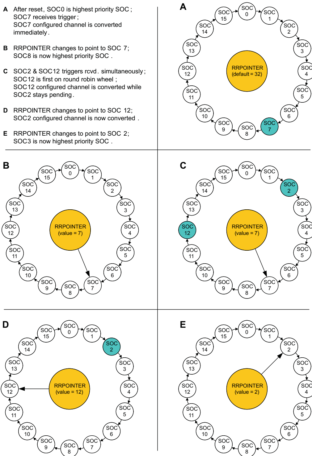
Figure 10-14. Round Robin Priority Example
