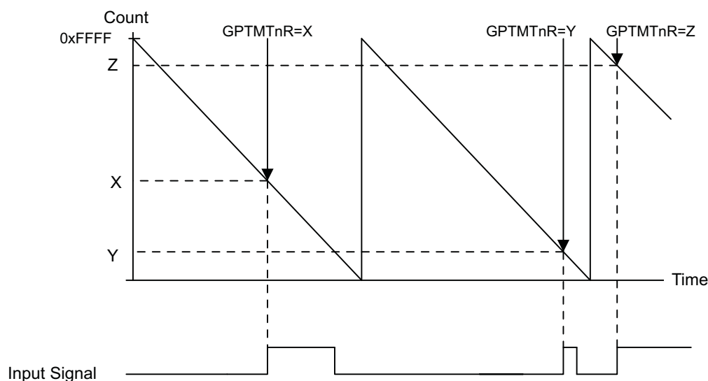
Figure 2-4. 16-Bit Input Edge-Time Mode Example
