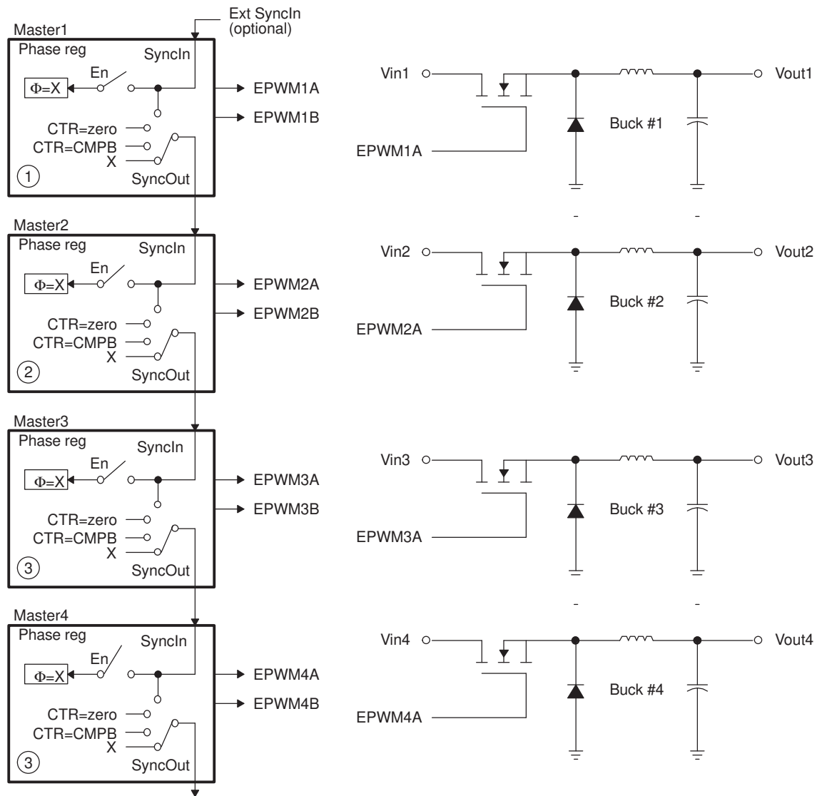
Figure 7-57. Control of Four Buck Stages. Here F_{PWM1} \neq F_{PWM2} \neq F_{PWM3} \neq F_{PWM4}
