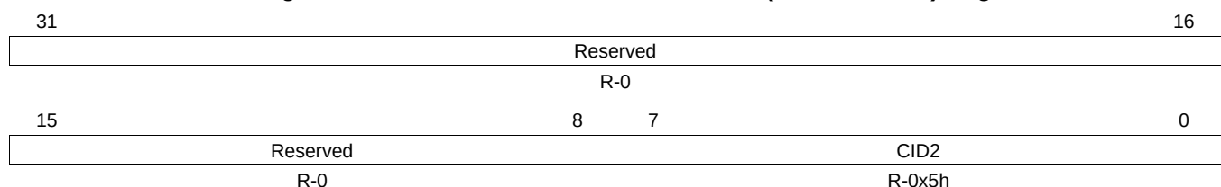
Figure 4-33. GPIO PrimeCell Identification 2 (GPIOCellID2) Register
