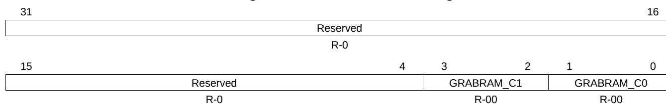
Figure 1-149. Z2_GRABRAMR Register
