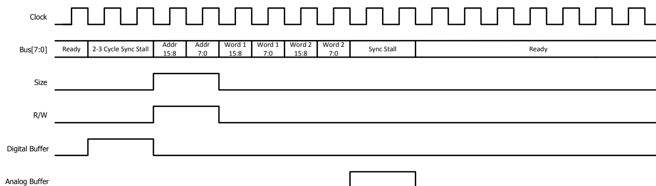
Figure 10-4. 32-bit Write
