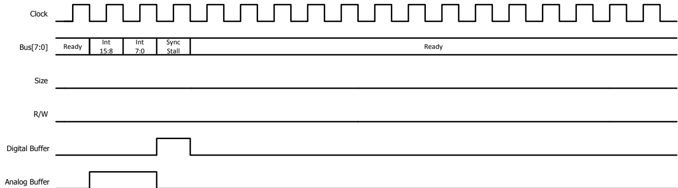
Figure 10-9. ADC Interrupt
