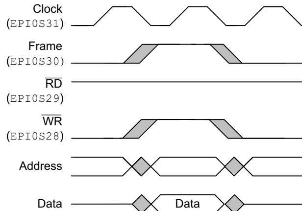
Figure 17-15. Single-Cycle Write Access, FRM50 = 0, FRMCNT = 0, WR2CYC = 0
