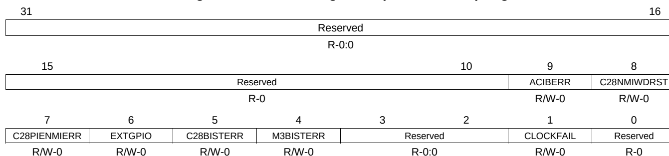
Figure 1-64. M3NMI Flag Force (NMIFLGFRFC) Register
