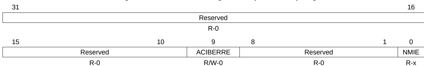
Figure 1-61. M3NMI Configuration (MNMICFG) Register
