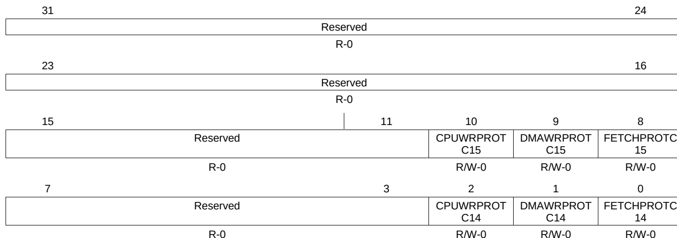
Figure 5-8. Cx SHRAM Configuration Register 4 (CxSRCR4)
