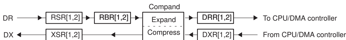
Figure 15-2. McBSP Data Transfer Paths
