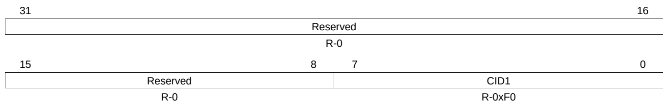
Figure 4-32. GPIO PrimeCell Identification 1 (GPIOCellID1) Register
