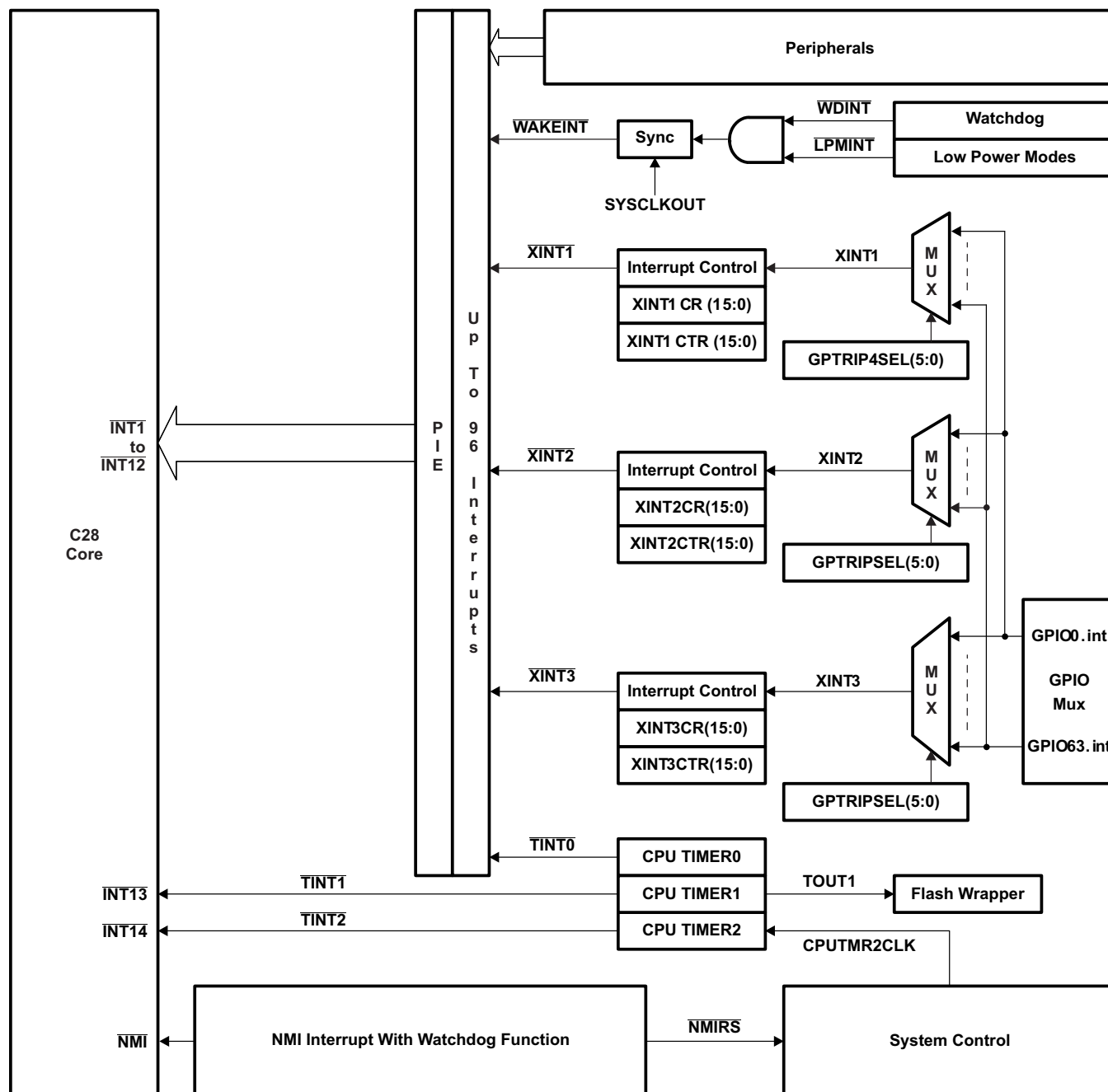
Figure 1-7. PIE Interrupt Sources and External Interrupts XINT1/XINT2/XINT3
