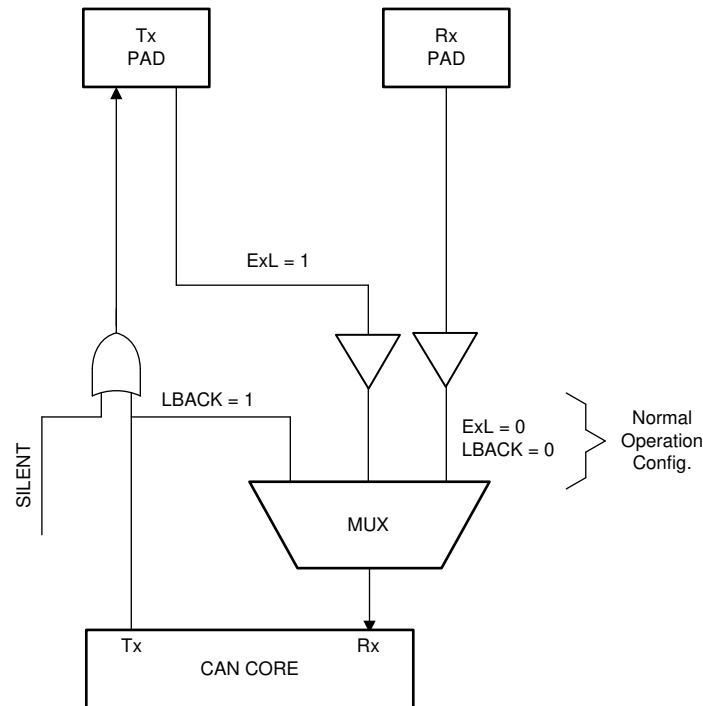
Figure 23-2. CAN_MUXing
