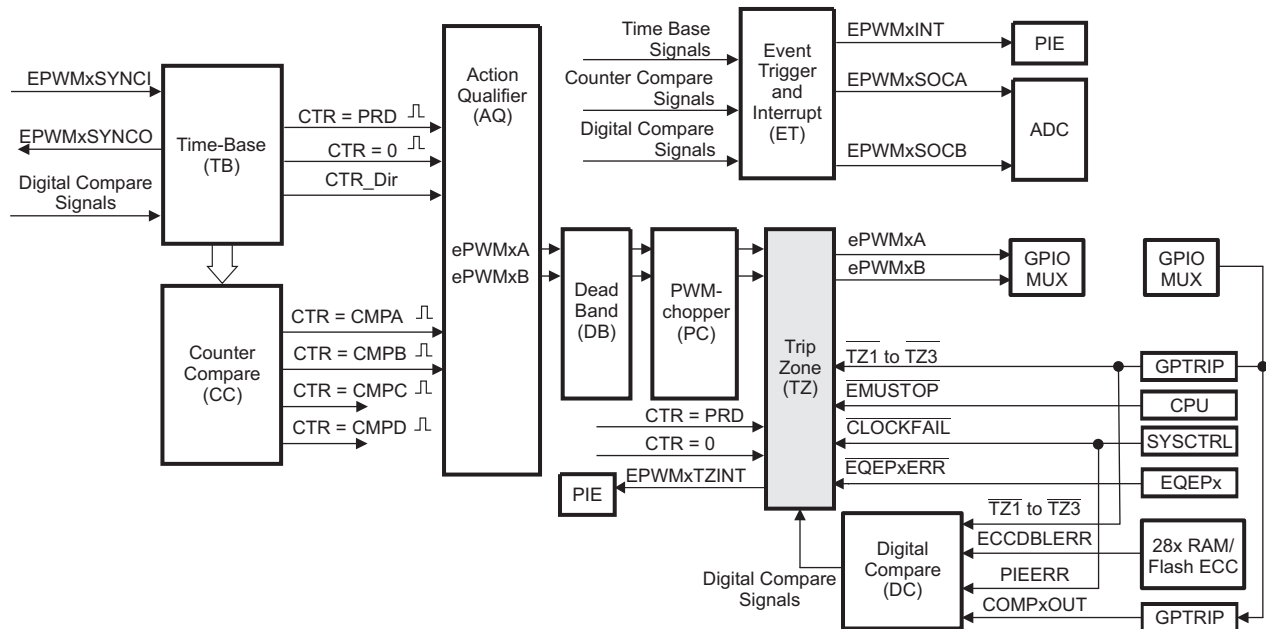
Figure 7-38. Trip-Zone Submodule
