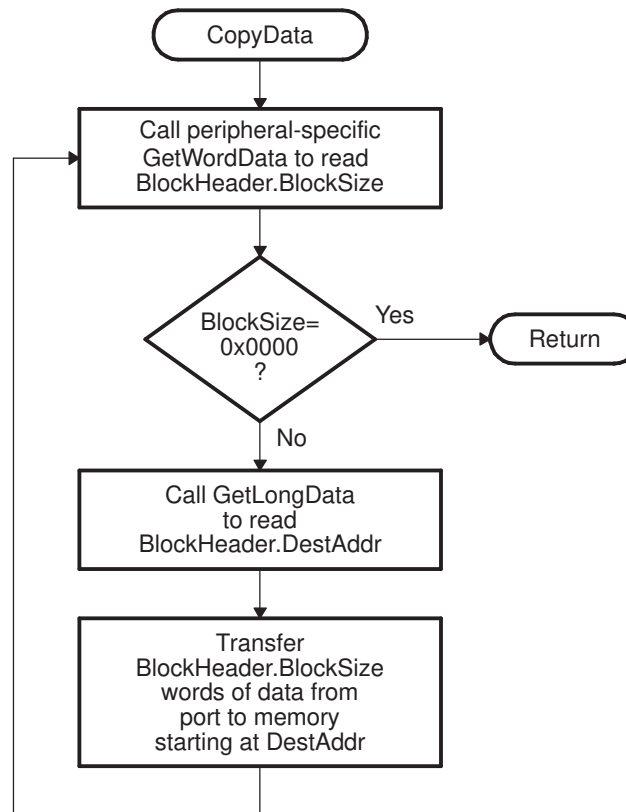
Figure 6-16. Overview of CopyData Function
