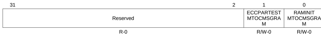
Figure 5-15. MTOC_MSG_RAM Test and Initialization Register (MTOCRTESTINIT)
