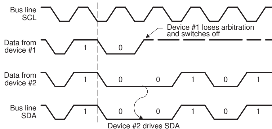
Figure 14-12. Arbitration Procedure Between Two Master-Transmitters
