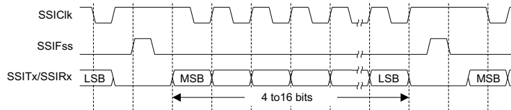
Figure 20-8. Freescale SPI Frame Format (Continuous Transfer) with SPO=1 and SPH=0
