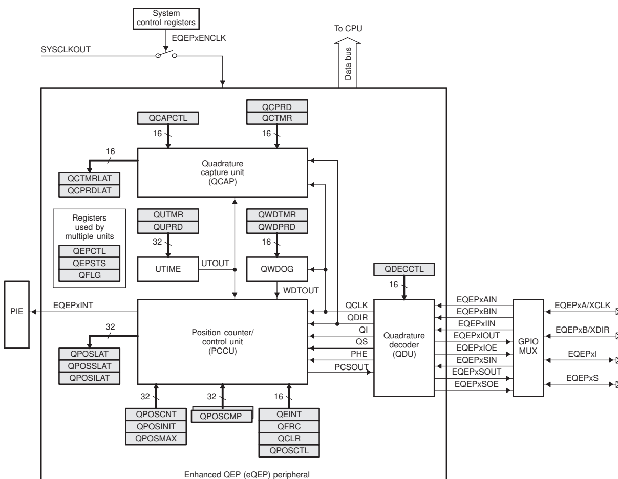
Figure 9-4. Functional Block Diagram of the eQEP Peripheral
