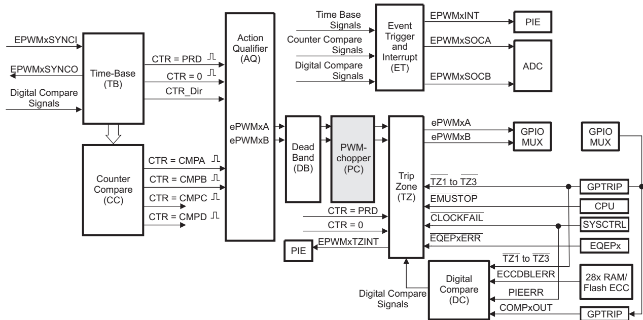
Figure 7-33. PWM-Chopper Submodule
