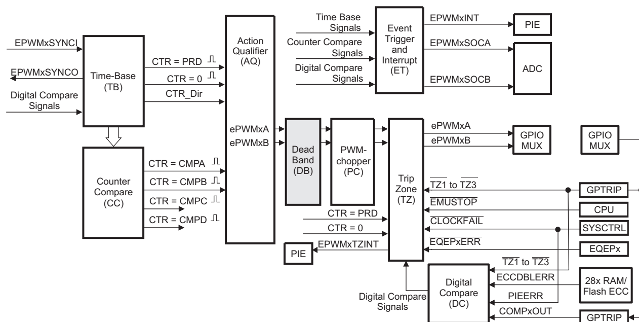
Figure 7-30. Dead_Band Submodule
