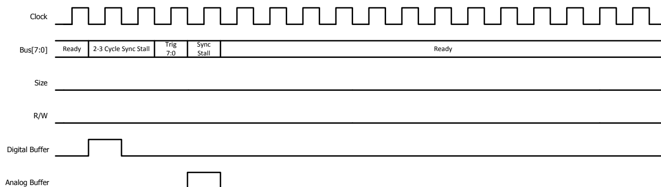
Figure 10-8. ADC Trigger
