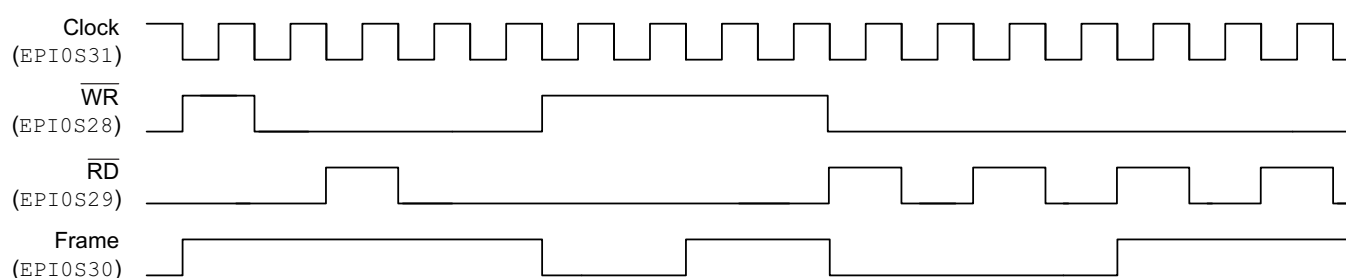
Figure 17-22. FRAME Signal Operation, FRM50 = 1 and FRMCNT = 1
