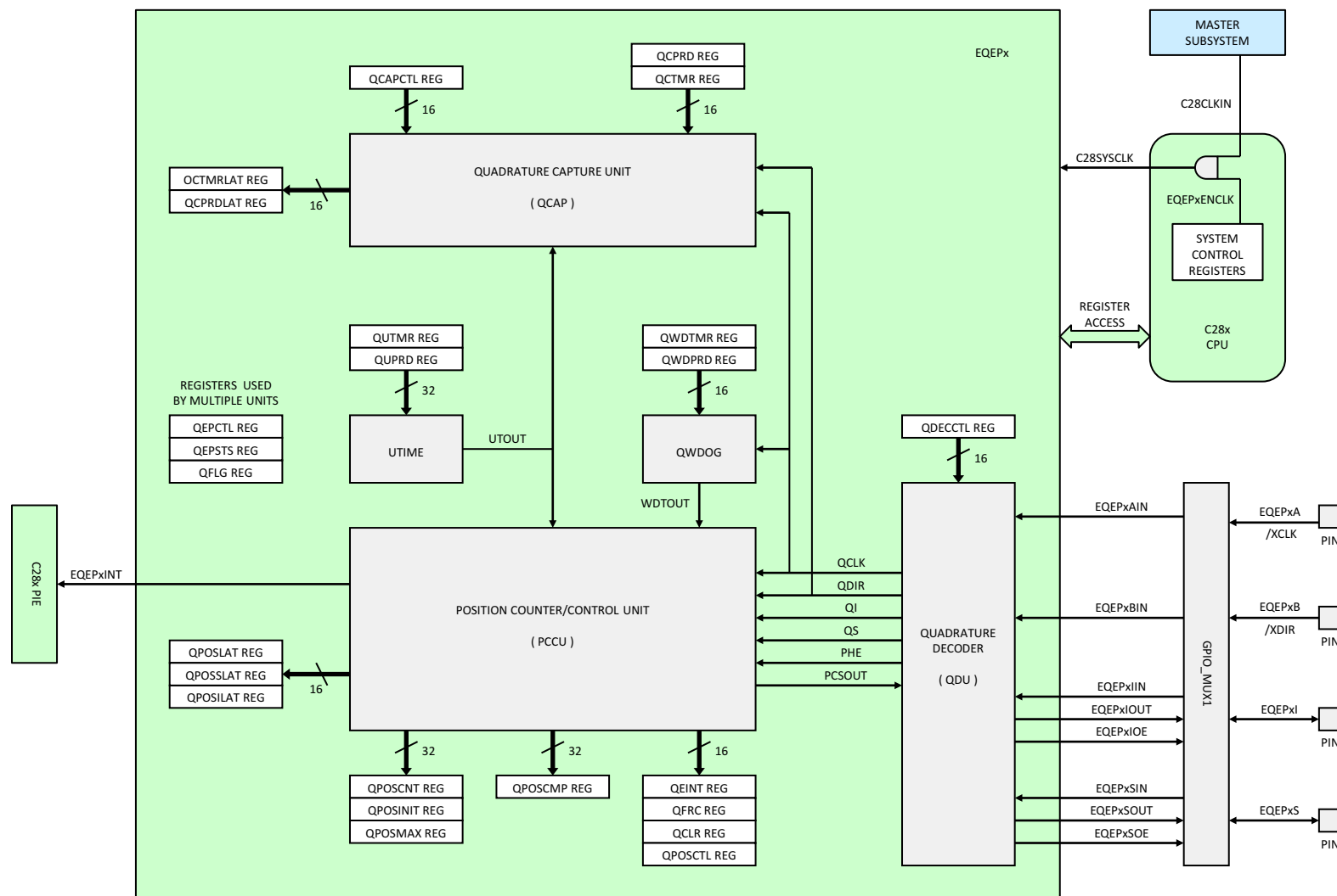
Figure 5-47. eQEP
