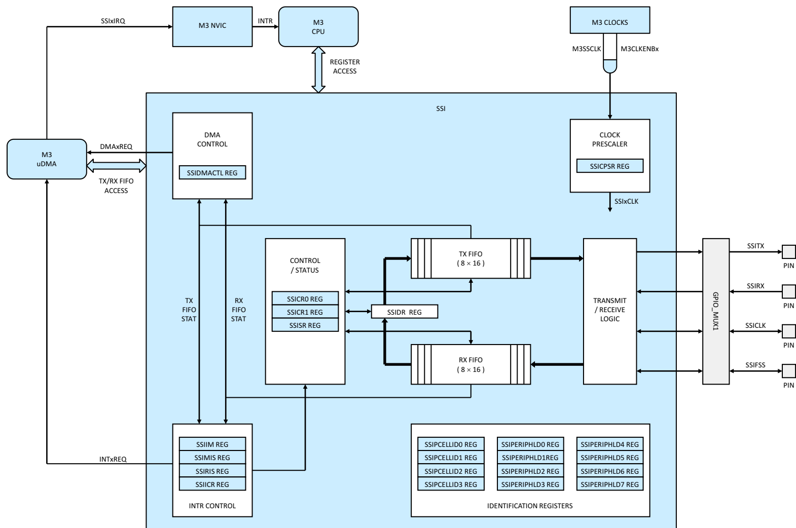
Figure 5-30. SSI
