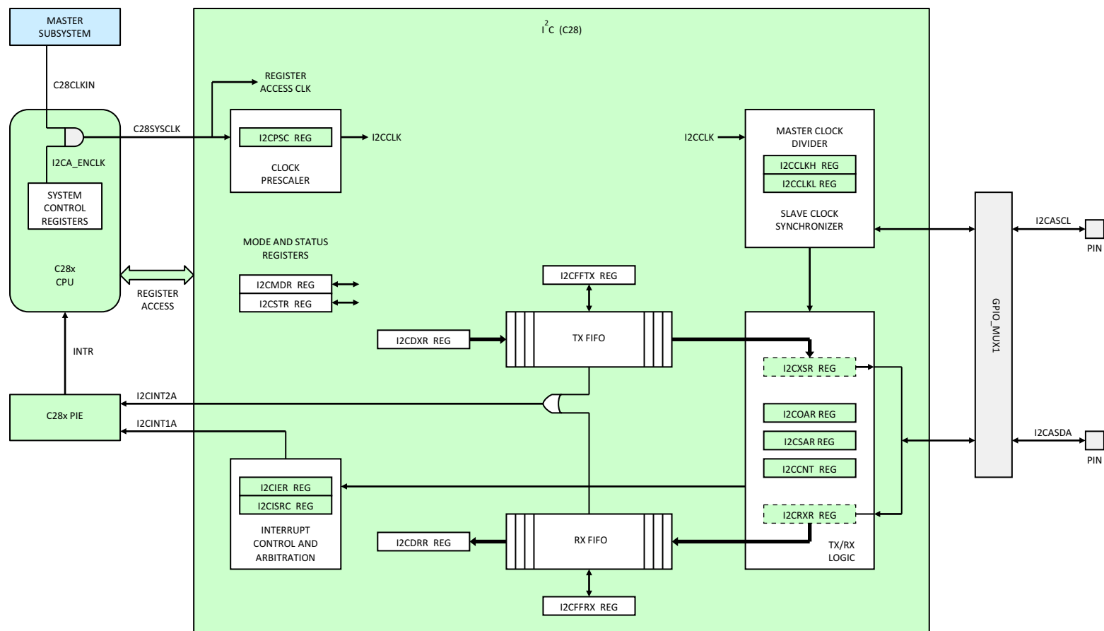
Figure 5-48. I2C (C28x)
