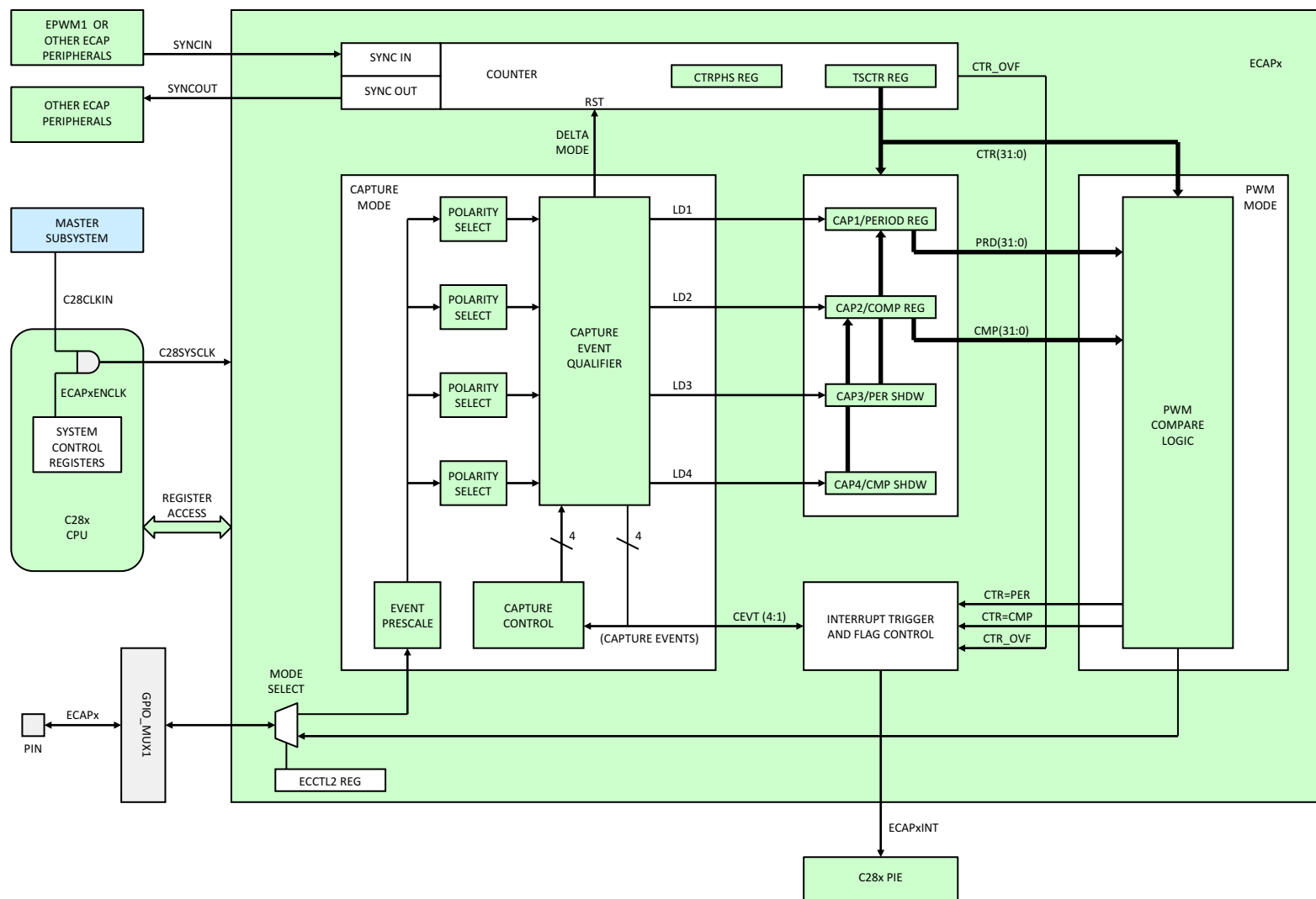
Figure 5-46. eCAP
