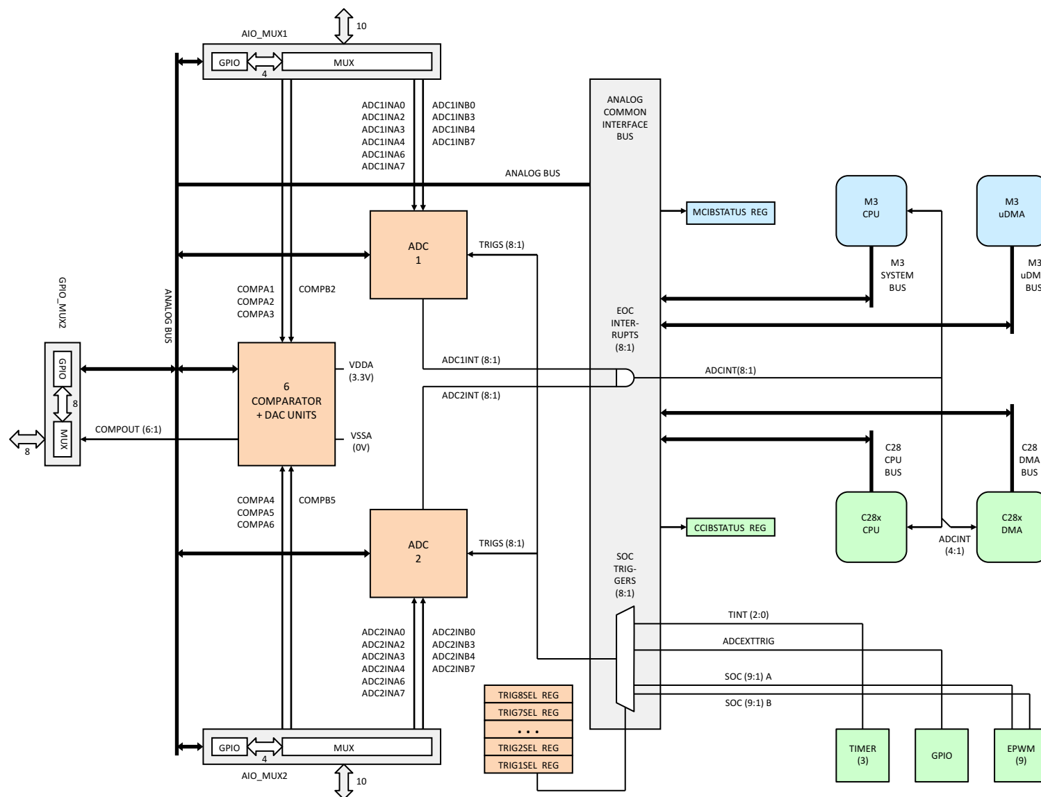
Figure 6-3. Analog Subsystem
