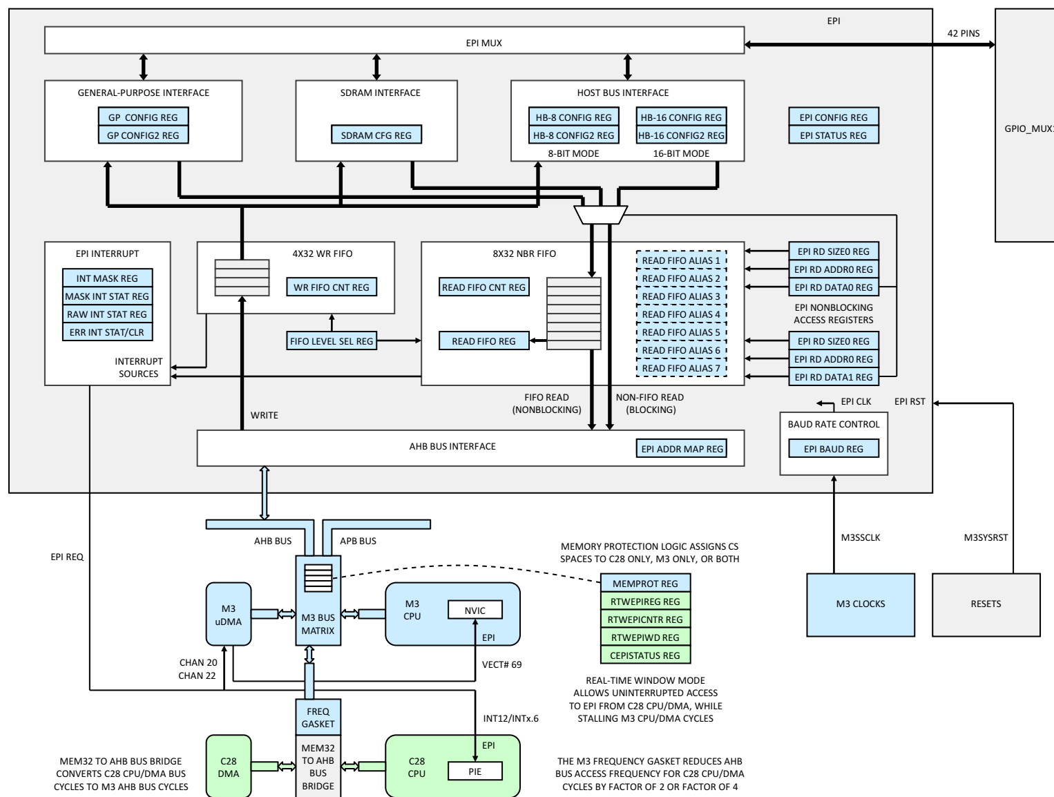
Figure 5-16. EPI
