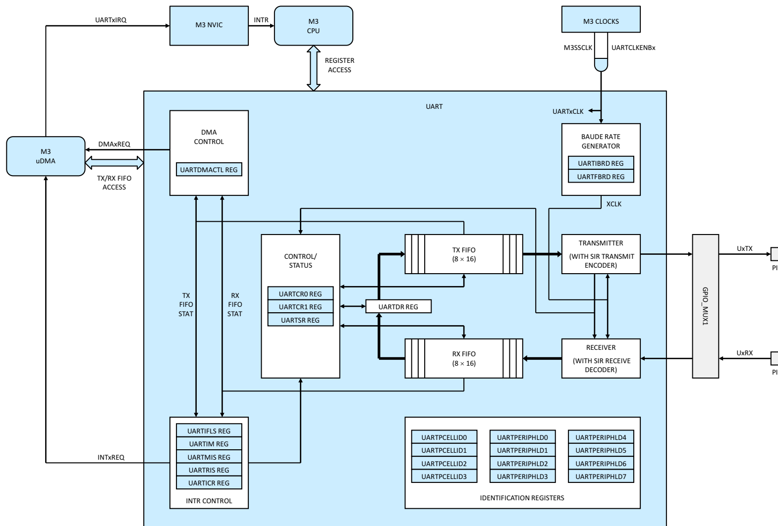
Figure 5-31. UART
