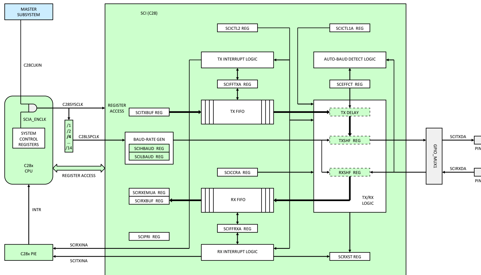
Figure 5-49. SCI (C28x)
