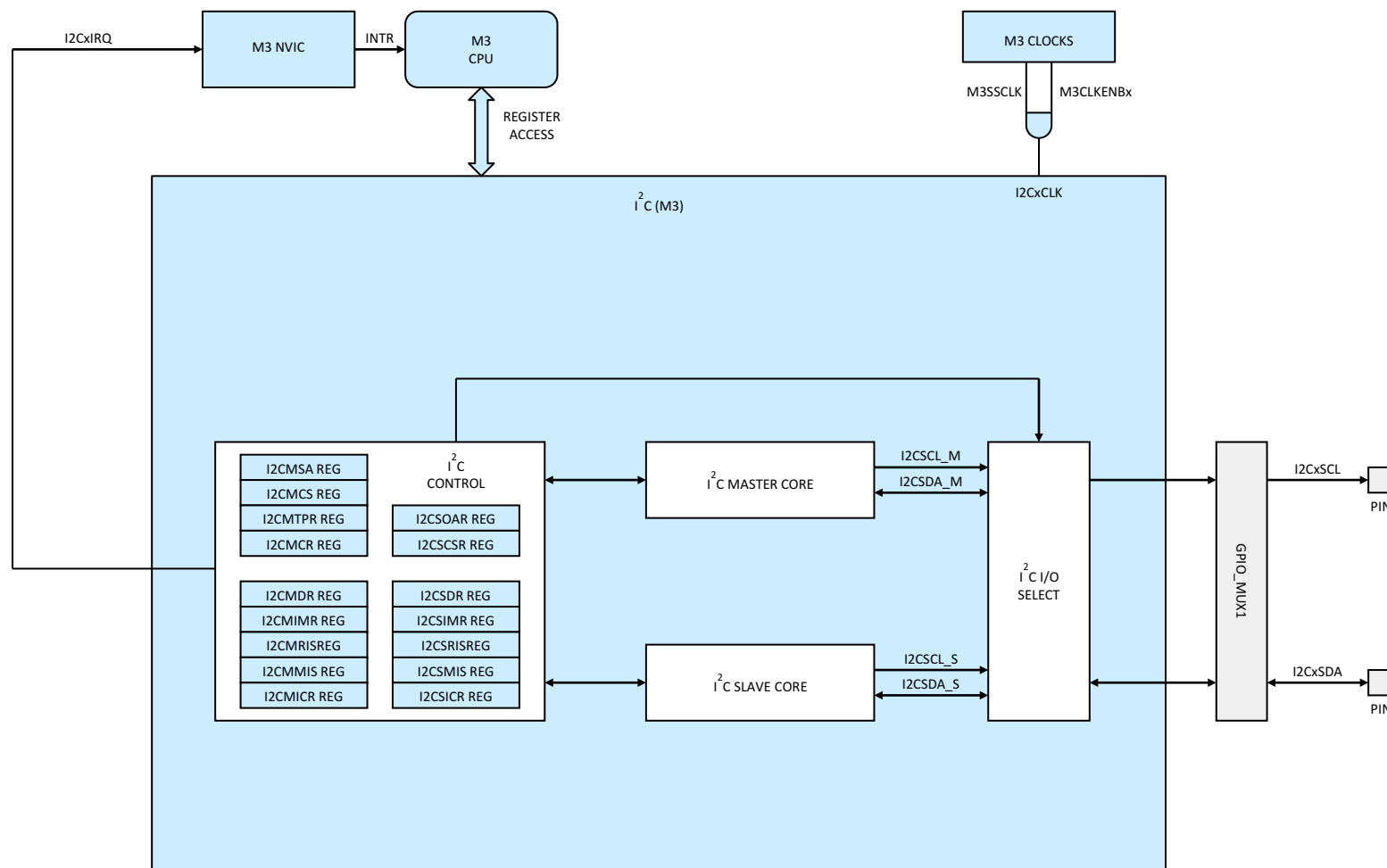
Figure 5-32. I2C (Cortex-M3)
