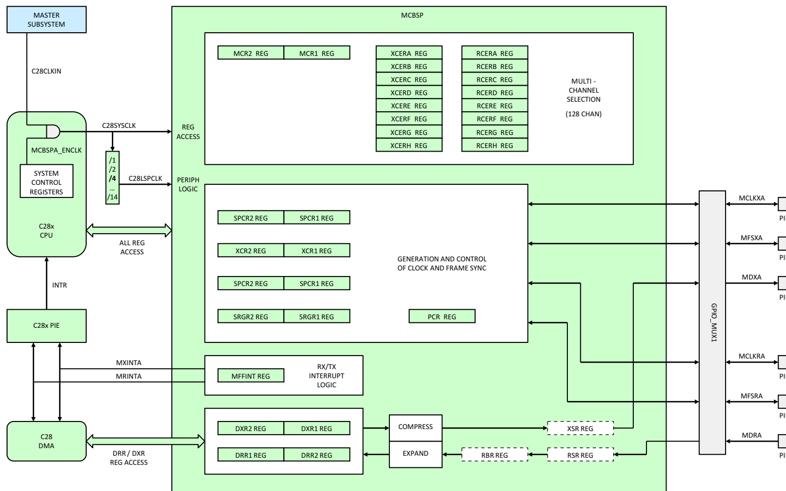
Figure 5-55. McBSP (C28x)
