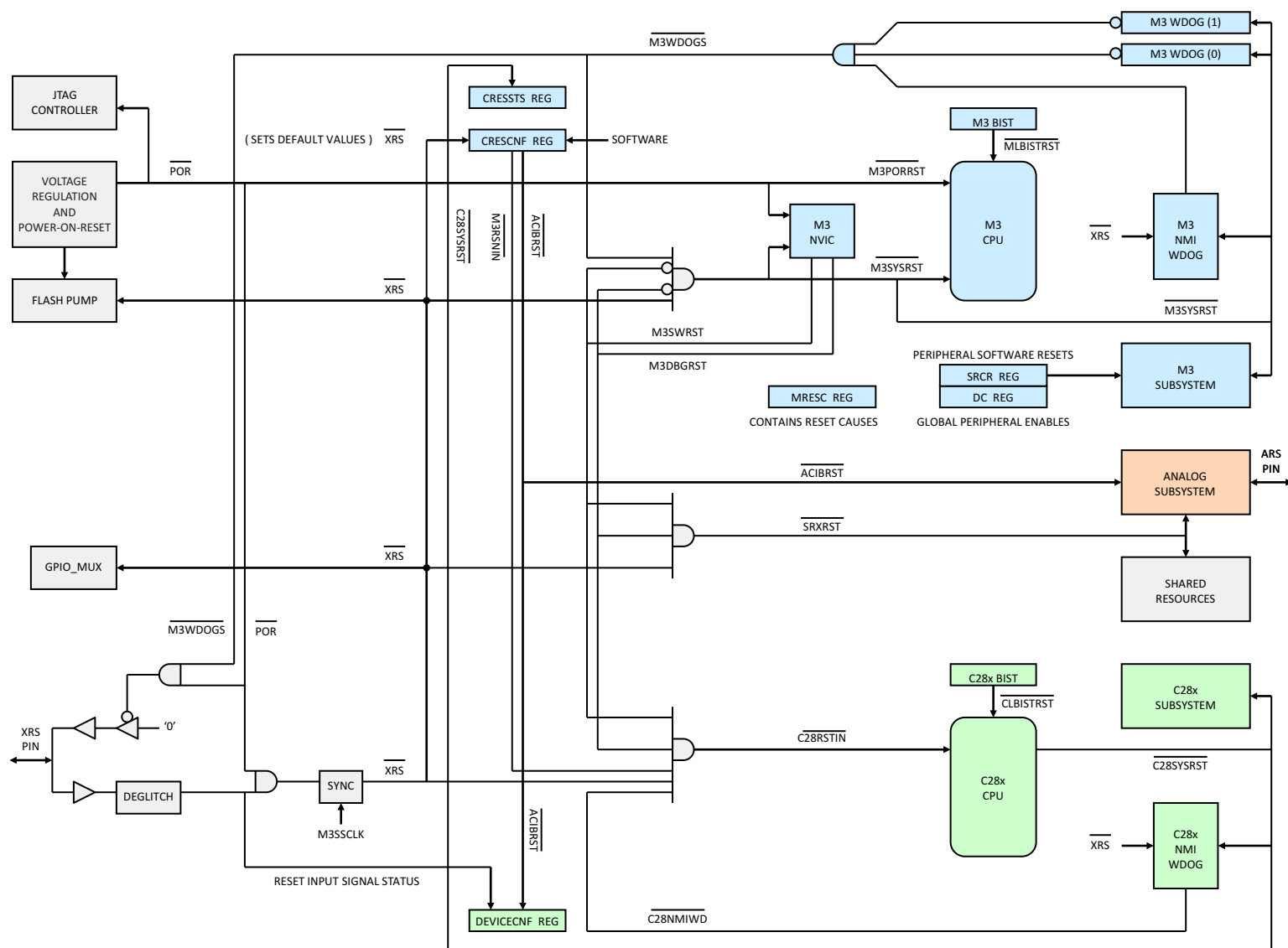
Figure 6-5. Resets
