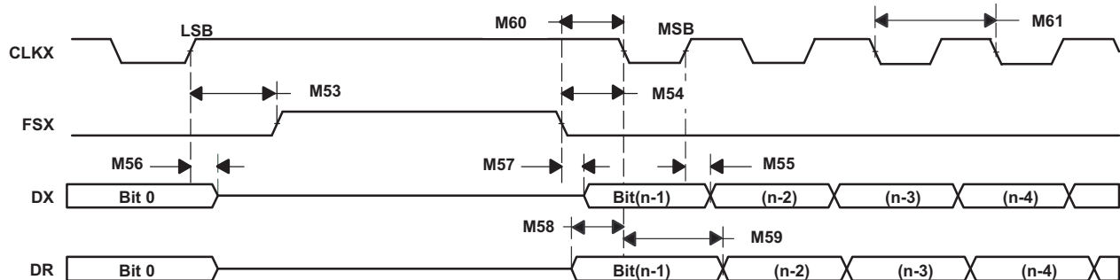
Figure 5-61. McBSP Timing as SPI Master or Slave: CLKSTP = 11b, CLKXP = 1
