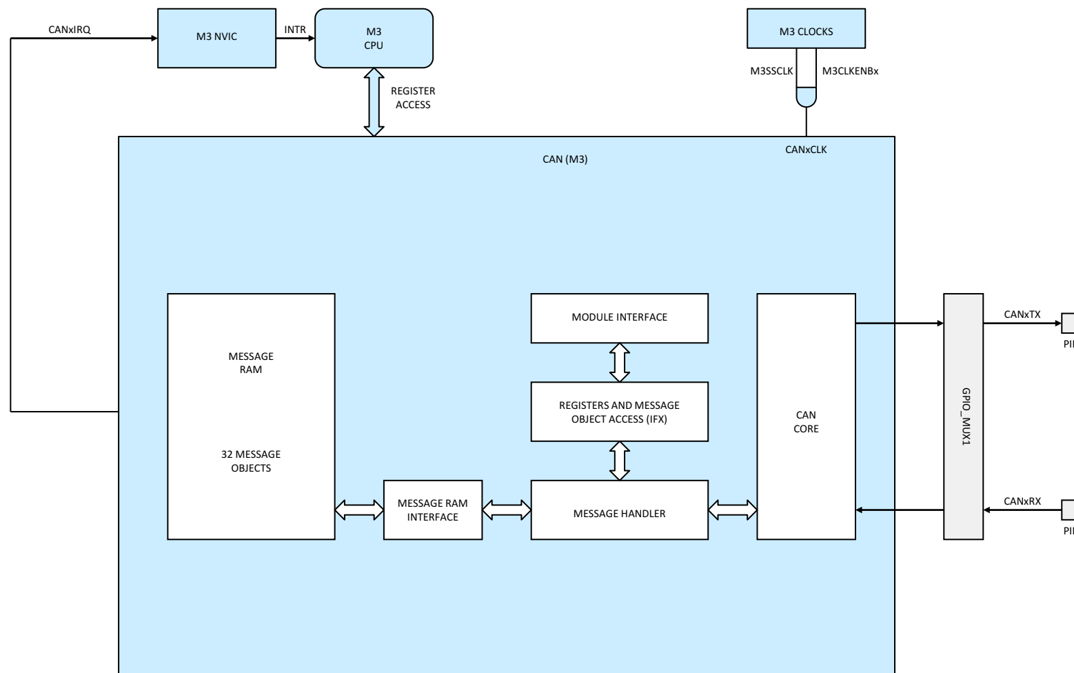
Figure 5-33. CAN (Cortex-M3)
