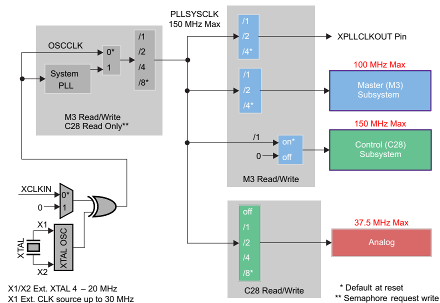
Figure 6-11. System Clock/PLL
