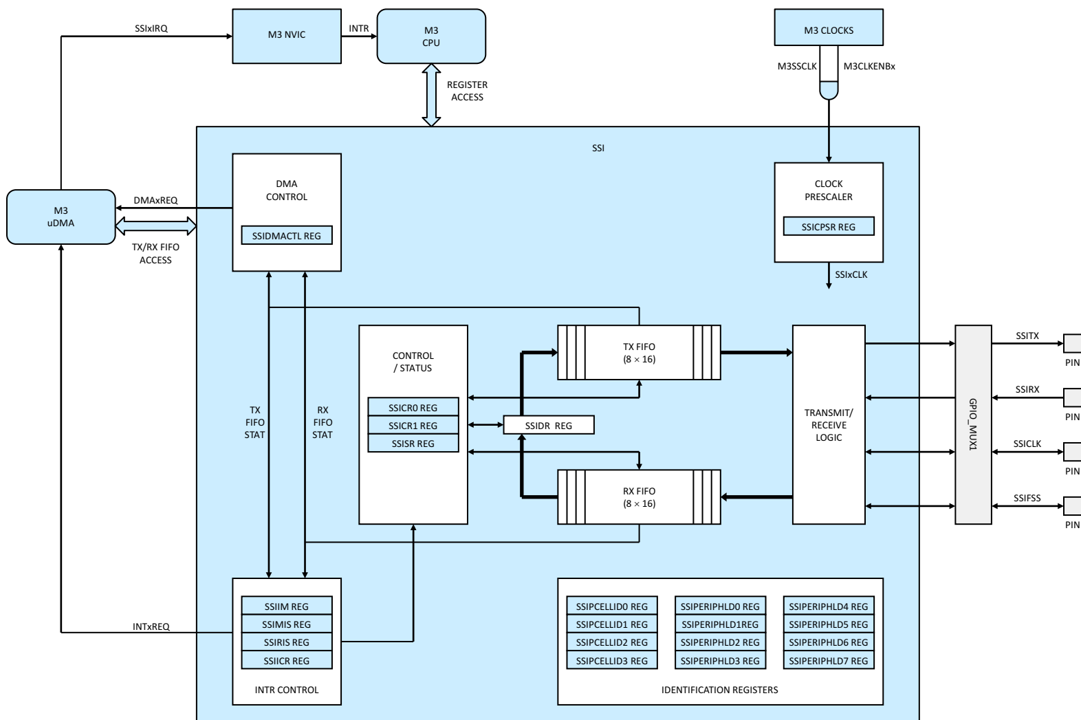
Figure 5-30. SSI
