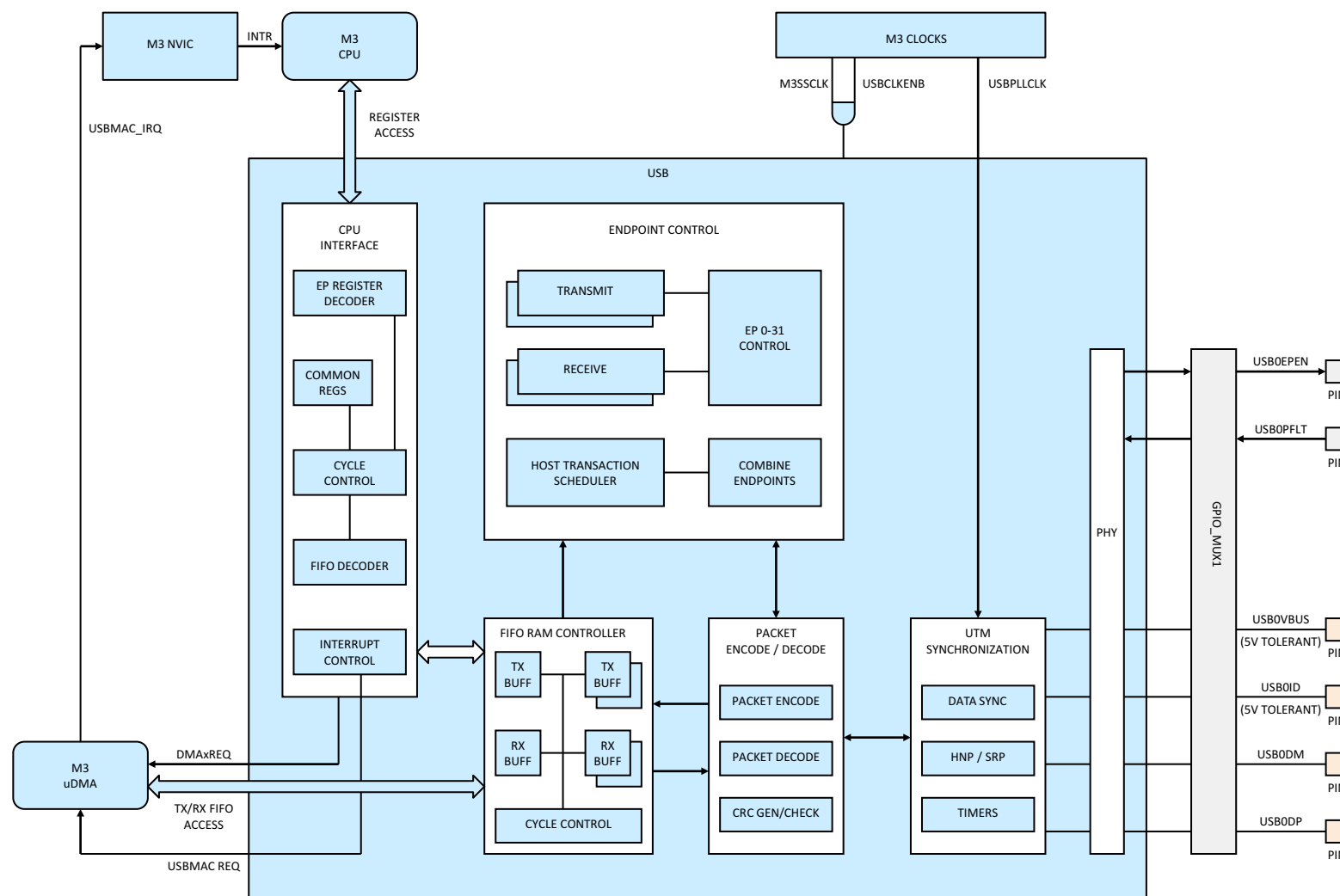
Figure 5-34. USB
