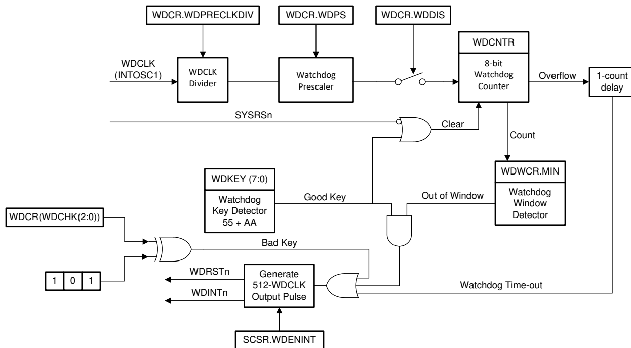
Figure 8-8. Windowed Watchdog
