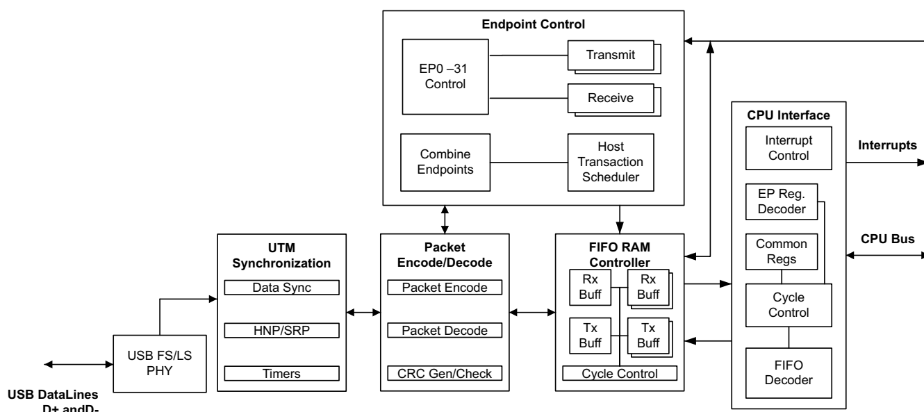
Figure 7-88. USB Block Diagram
