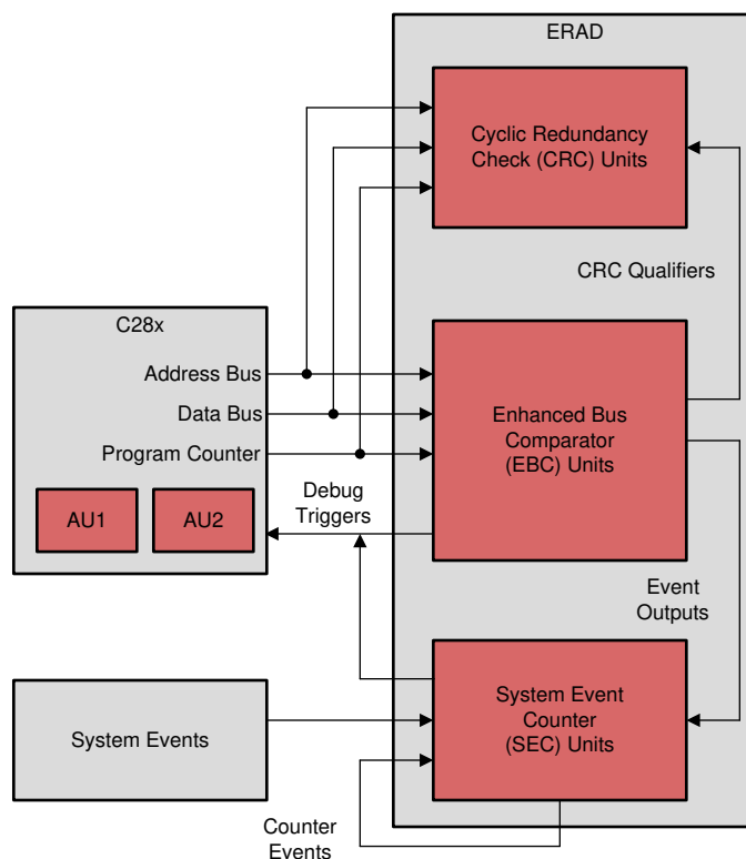
Figure 8-2. ERAD Overview
