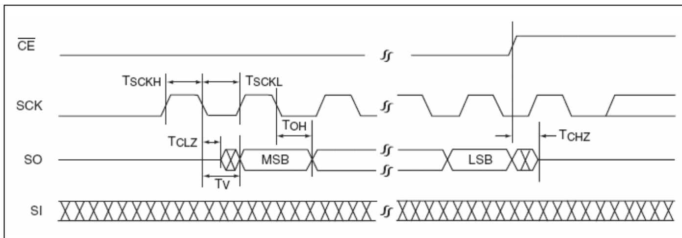
Figure 21: Serial Output Timing Diagram
