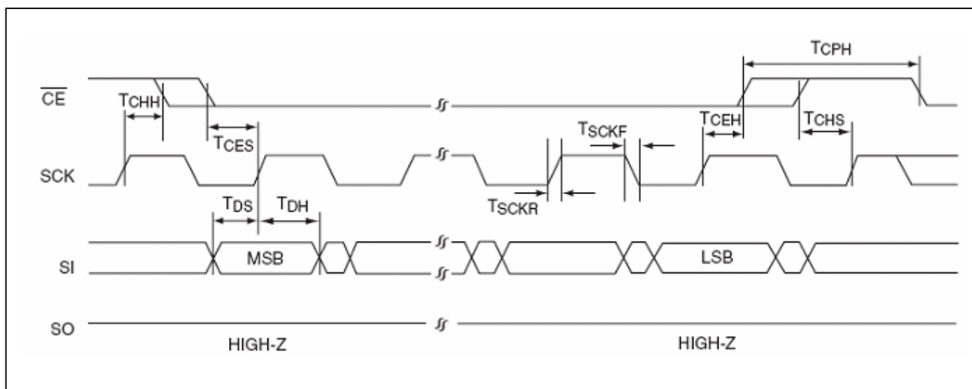
Figure 20: Serial Input Timing Diagram
