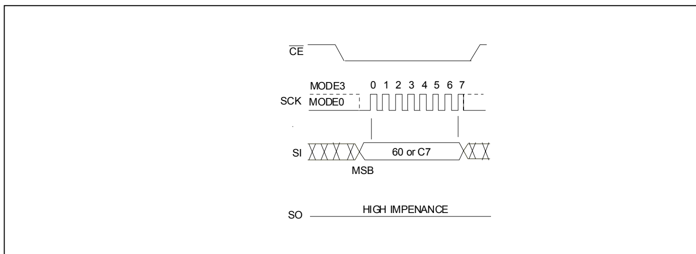
FIGURE 7 : CHIP-ERASE SEQUENCE
