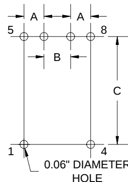
Board Layout
